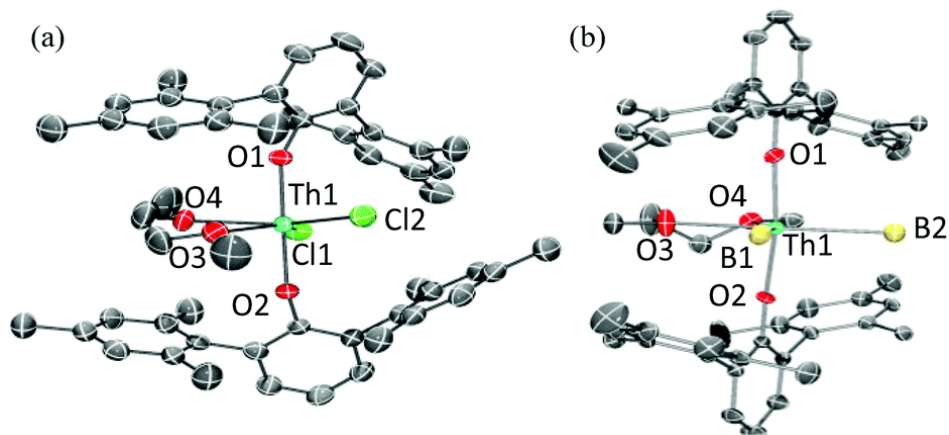
Figure 1. Displacement ellipsoid drawing of the solid-state molecular structure of 1a (left) and 1b (right) (50 % probability ellipsoids). Hydrogen atoms, solvent molecules and disorder in DME molecule are omitted for clarity.
