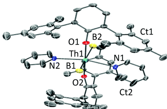
Figure 3. Displacement ellipsoid drawing of the solid-state molecular structure of the monomeric unit of 3 (50 % probability ellipsoids). Hydrogen atoms and toluene solvent molecules are omitted for clarity.
