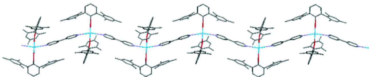
Figure 5. A portion of the 1-D polymeric chain structure of 3 . Hydrogen atoms and toluene solvent molecules removed for clarity.
