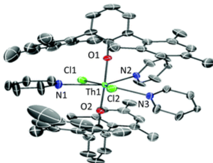
Figure 4. Displacement ellipsoid drawing of the solid-state molecular structure of the monomeric unit of 4 (50 % probability ellipsoids). Hydrogen atoms and lattice benzene and bipyridine molecules removed for clarity.
