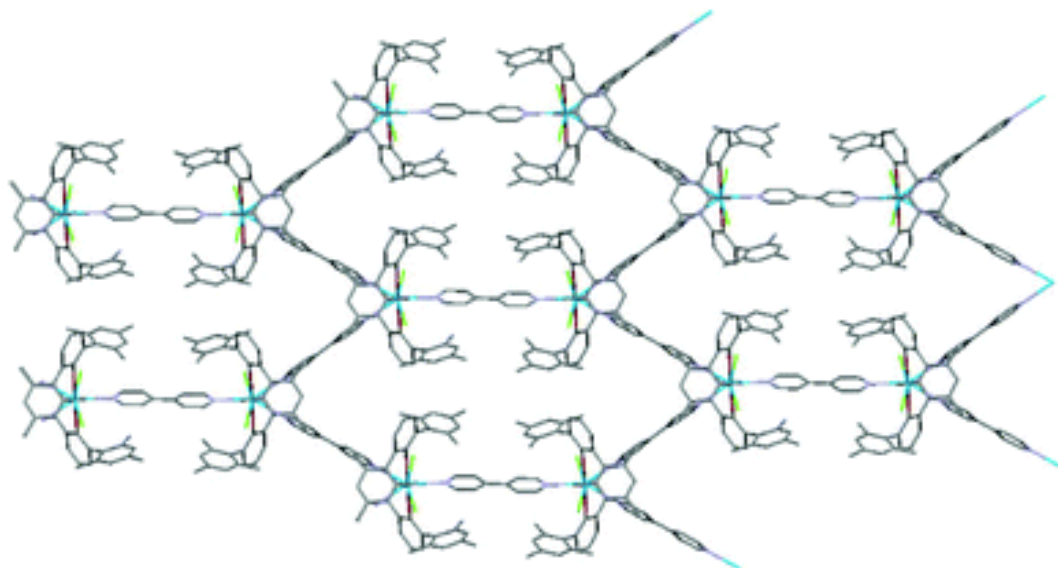
Figure 6. A portion of the 2-D polymeric chain structure of 4 . Hydrogen atoms and lattice benzene and bipyridine molecules removed for clarity.
