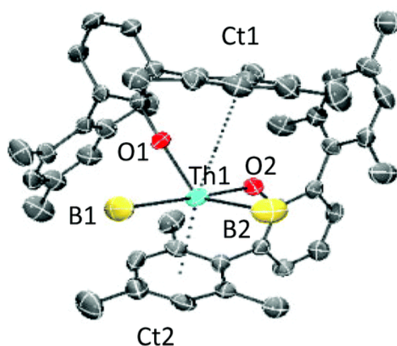
Figure 2. Displacement ellipsoid drawing of the solid-state molecular structure of 2 (50 % probability ellipsoids). Hydrogen atoms are omitted for clarity.
