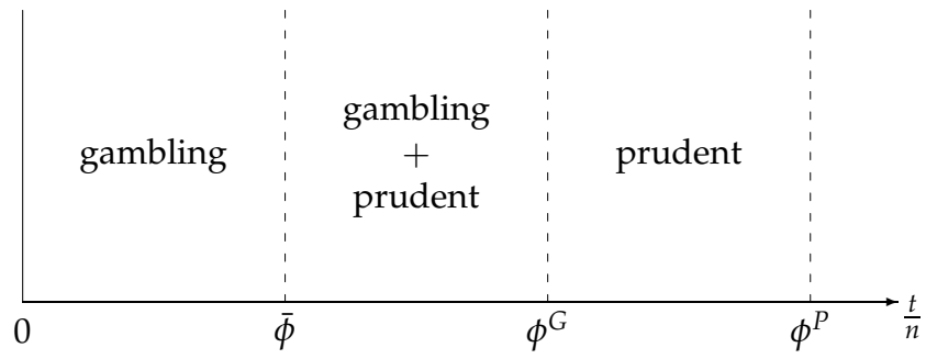
Figure 1: Characterisation of equilibria
