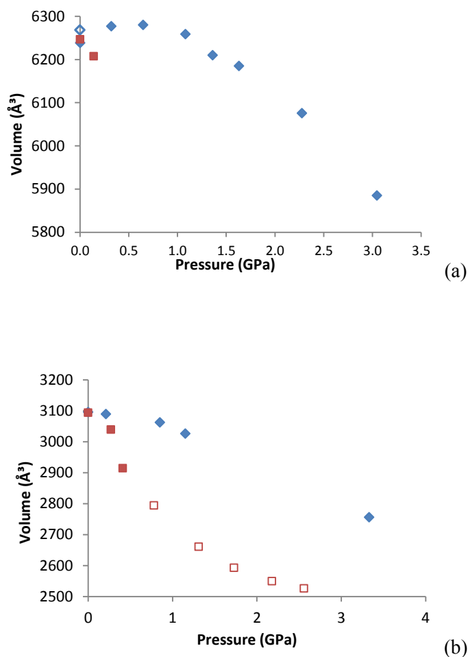
Figure 3. Unit cell volume of (a) Sc 2 BDC 3 and (b) Sc 2 (NO 2 -BDC) 3 in methanol (blue diamonds) and Fluorinert FC-77 (red squares) as a function of pressure. In (a) the open blue diamond refers to the ambient structure surrounded with MeOH in a capillary. In (b) the closed and open red squares refer to the C2/c and Fdd2 structures respectively, with the unit cell halved for the latter. Error bars are smaller than the symbols.
