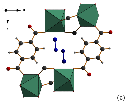
Figure 1. (a) Triangular pores formed in \text{Sc}_2\text{BDC}_3 viewed along the a -axis. Disordered methanol molecules are represented by solid red (Site 1) and blue (Site 2) coloured molecules. Openings between triangular channels of \text{Sc}_2\text{BDC}_3 between (b) Group 1 and (c) Group 2 ligands as viewed along the c and b -axes, respectively. Key: C, grey; \text{ScO}_6 octahedra, green; O, red; H, light grey.
