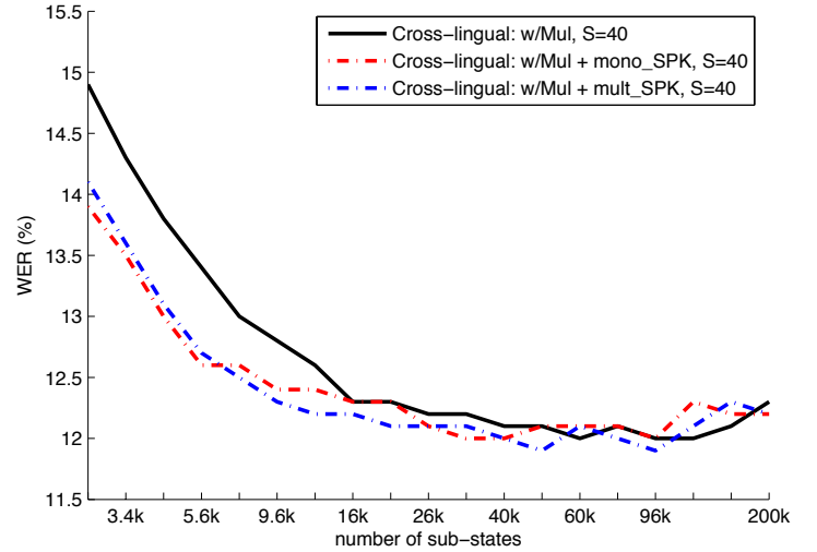
Fig. 14. WER of cross-lingual systems using speaker subspace, 15h training data, tested on the development dataset.
