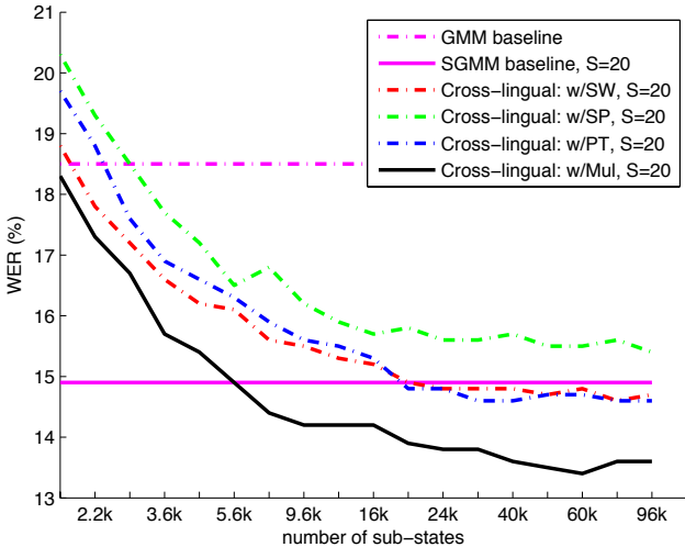
Fig. 5. WER of baseline cross-lingual systems, 5h training data, tested on the development dataset. Only the lowest WER of SGMM baseline system by tuning the number of sub-states is given for clarity.
