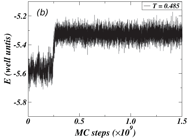
Figure 5. (a) Specific heat as function of temperature for a confined L-J system with N = 515 particles and an effective filling fraction \phi \simeq 45\% . Zooms of the specific heat is represent in the inset. (b) Energy sampling for the same system during a full MC run at a temperature T = 0.485 , corresponding to a phase-switching region.
