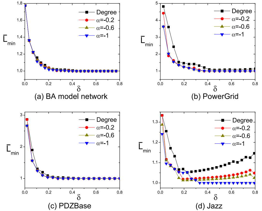
Figure 6. The average shortest distance \bar{L}_{min} as a function of \delta and \alpha for four network at C = 10 . Note that, large-degree pinning control ( Degree ) where the pinning nodes are got by selecting the largest \lfloor N\delta \rfloor degree nodes.
