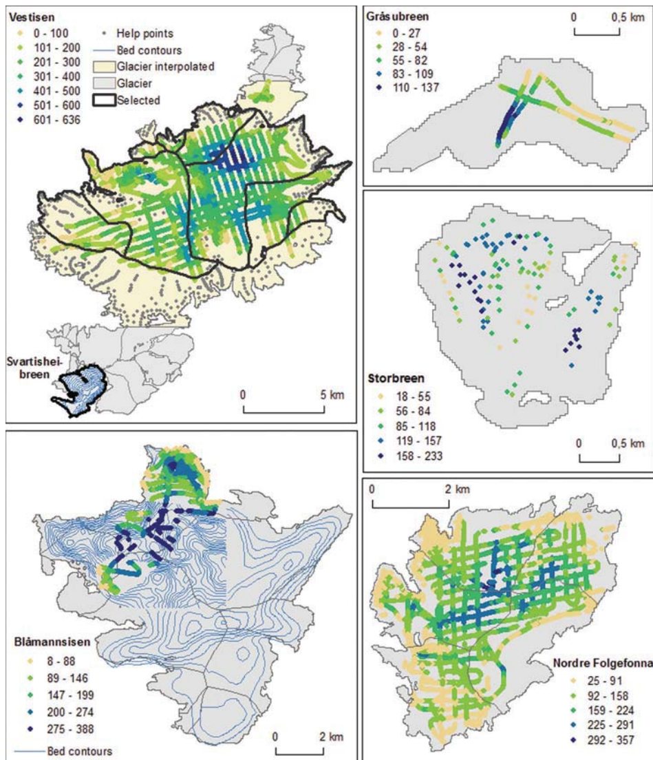
Fig. 2. Examples of various ice thickness data: Vestisen (SVV), Blåmannsisen (BLÅ), Grås ubreen (2743), Storbreen (2636) and Nordre Folgefonna (NFF). See Figure 1 for locations. Vestisen has been measured in several campaigns, and bed contours are available for Svartisheibreen. Ice thickness of Blåmannsisen was derived from interpolated bed contours made from campaigns in 1989 covering large parts of the glacier and additional measurements of Rundvassbreen in 2004. At Grås ubreen, three profiles were collected in fall 2012. At Storbreen, point measurements were collected in 2005 and 2006. At Nordre Folgefonna, dense measurements were performed in 2012.
