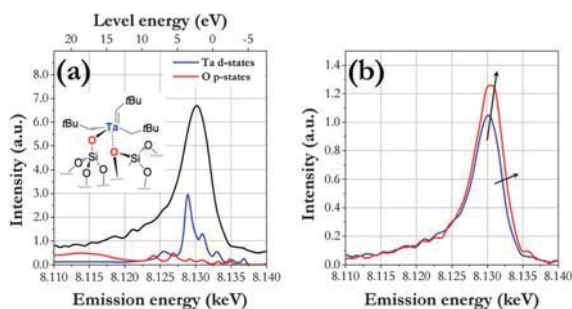
Fig. 1 (a) HEROS spectrum (black) and calculated density of unoccupied Ta d- and O p-states for [(\equiv\text{SiO}_2)\text{Ta}(=\text{CHtBu})(\text{CH}_2\text{tBu})_2] . The level energy scale on the top axis refers only to the presented DOS and shows its distribution around the Fermi level. (b) Comparison between the HEROS spectra of [(\equiv\text{SiO}_2)\text{Ta}(=\text{CHtBu})(\text{CH}_2\text{tBu})_2] (blue) and [(\equiv\text{SiO}_2)\text{TaH}_3] (red).
