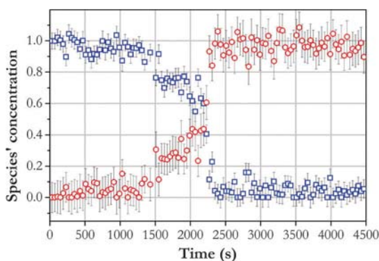
Fig. 5 Spectral evolution as a function of time on stream. The data was fitted with two components (□) [(\equiv \text{SiO}_2)\text{Ta}(\text{=CHtBu})(\text{CH}_2\text{tBu})_2] ; (○) after oxidation.
