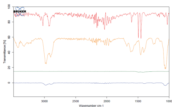
Fig. S2 FTIR spectra of polystyrene nanospheres (red), \text{AgNP}/\text{PS} coated with \text{CeO}_2 (yellow), \text{AgNP}/\text{CeO}_2 capsules obtained by calcination (green), and \text{AgNP}/\text{CeO}_2 capsules obtained by dissolution (blue).
