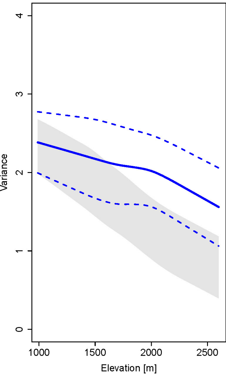
(a) Variance in proboscis length, sc. A2 2085
