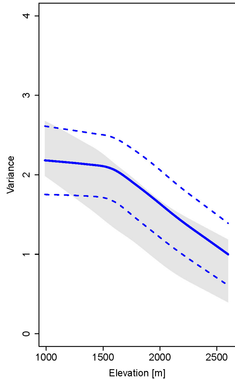
(c) Variance in proboscis length, sc. RCP3PD 2085
