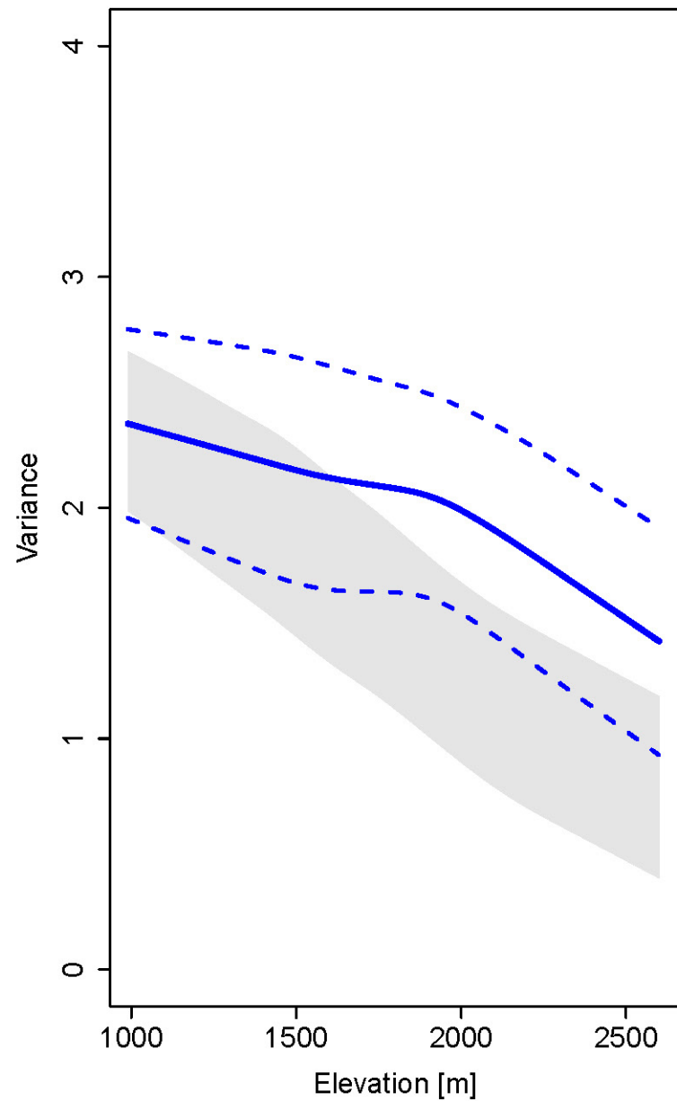
(b) Variance in proboscis length, sc. A1B 2085
