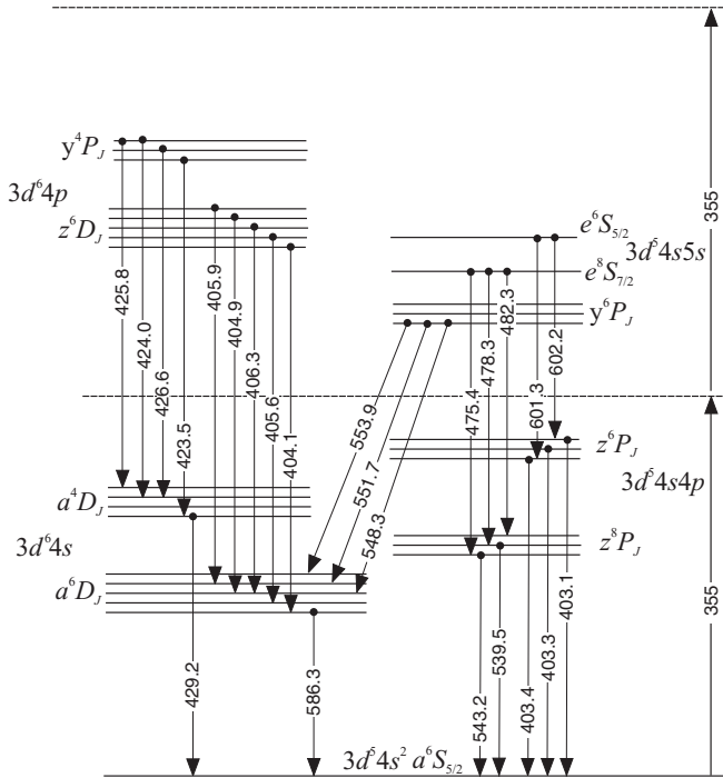
FIG. 1. Electronic states and transitions of Mn atom. 8 Because of the very large number of excited states, only the states discussed in the present work are shown. Horizontal dashed lines indicate the energies accessible by one-photon and two-photon excitation at \lambda = 355 nm. Transition wavelengths are given in nm.
