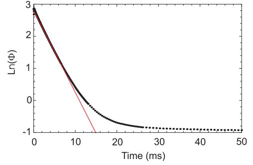
FIG. 5. Autocorrelation function of the luminescence signal at \lambda = 586 nm following an excitation pulse at t=0 . Dots: experimental data; solid line: fitted exponential decay.
