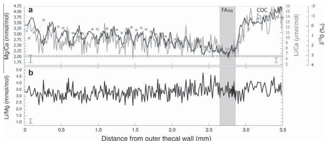
Fig. 2. (a) Li/Ca (grey line) and Mg/Ca (black line) ratios from laser ablation ICP-MS along the thecal wall of a specimen of Lophelia pertusa collected in Propeller Mound (sample POS-265-499), together with micro-scale variations in the oxygen isotope composition (grey dots) of micro-milled subsamples. (b) Li/Mg ratios along the same transect. Grey bar represents the portion of fibrous aragonite precipitated closest to the expected isotopic equilibrium with ambient seawater (FA eq ). COCs: centres of calcification. Horizontal thick and dotted lines represent expected isotopic equilibrium with ambient seawater ( \delta^{18}\text{O}_{\text{eq}} = 2.8 \pm 0.2\text{‰} ).
