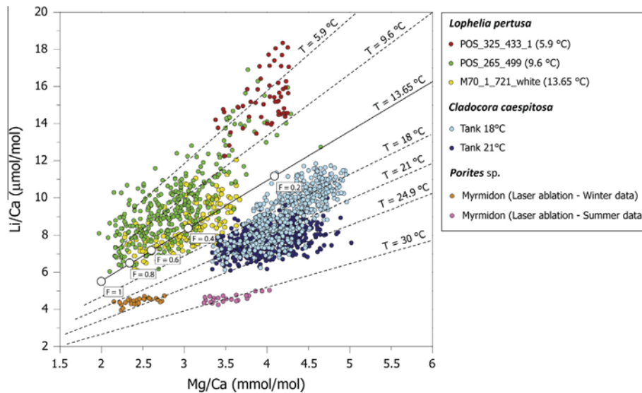
Fig. 7. Laser ablation ICP-MS Li/Ca and Mg/Ca values for specimens of L. pertusa , C. caespitosa and Porites sp. plotted together with calculated Rayleigh model lines. Values for L. pertusa and C. caespitosa represent fibrous aragonite. F is the fraction of Ca remaining in the parent solution. Our results show that the Rayleigh fractionation model can explain most of the fine-scale Mg/Ca versus Li/Ca variations observed in tropical, temperate and cold-water corals. However, the scatter of Li/Ca and Mg/Ca (and thus Li/Mg ) for small local temperature variations points towards an additional influence on Li/Mg ratios, which must be independent of the fraction of aragonite secreted by the organism. As mentioned above, the partition coefficients for Li/Ca and Mg/Ca positively correlate with growth rate in corals and inorganically-precipitated aragonite, suggesting that both ratios are influenced to some degree by crystal growth kinetics. However, the K_d 's for Li and Mg have different rate dependence, with the dependence of Mg/Ca being higher than that of Li/Ca (Gabitov et al., 2011). Therefore, the effect of this difference within the fibrous aragonite is not cancelled out when normalizing Li on Mg (Figs. 2b and 6) and a residual signal remains on the Li/Mg ratio that needs to be further investigated. Note that the difference in Li/Ca and Mg/Ca ratios between the fast-growing COCs and the surrounding fibrous aragonite due to crystal growth kinetics could overestimate the temperature reconstruction ( i.e. lower Li/Mg ). Therefore, the Li/Mg temperature proxy might not work in the presence of high amount of COCs ( e.g. along the septa of some coral species) or where large differences in growth rate occur.
