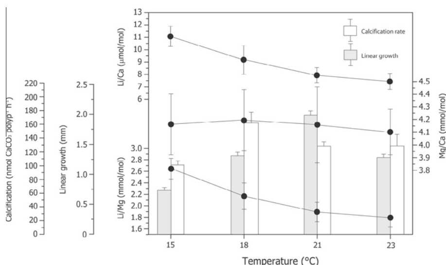
Fig. 3. Variations in Li/Ca, Mg/Ca and Li/Mg ratios compared to the calcification and linear extension rate of the coral skeleton of Cladocora caespitosa , cultured in experimental tanks at four different temperature conditions (15, 18, 21 and 23 °C). Linear extension rate increases as temperature increases from 15 °C to 21 °C but decreased by 36% at 23 °C compared to 21 °C. Calcification is variable among the temperature treatments, with corals maintained at 15 °C and 21 °C displaying lower and higher calcification rate, respectively. The Li/Ca ratios are inversely correlated to the water temperature of the tanks and display an exponential regression, whereas the values of Mg/Ca remain substantially constant within error. The resulting Li/Mg ratios decrease exponentially from 2.65 to 1.79 mmol/mol, and follow temperature.
