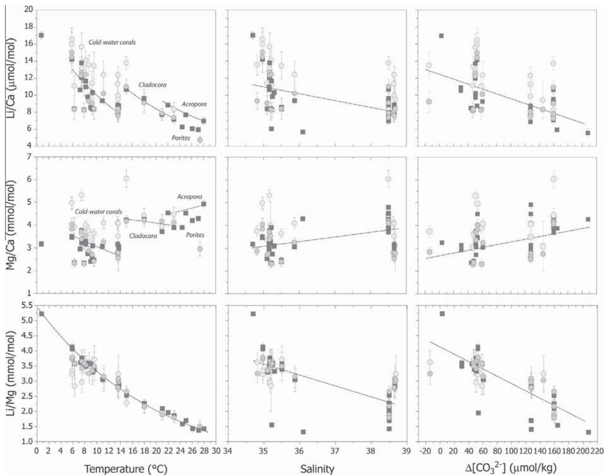
Fig. 5. Li/Ca, Mg/Ca and Li/Mg variations for cold-water, temperate and tropical corals related to changes in temperature, salinity and \Delta\text{CO}_3^{2-} . Grey and white circles represent laser ablation ICP-QMS values for fibrous aragonite and COCs, respectively. Note that for specimens of L. pertusa and M. oculata only values for \text{FA}_{\text{eq}} are plotted. Black squares represent solution ICP-MS data.
