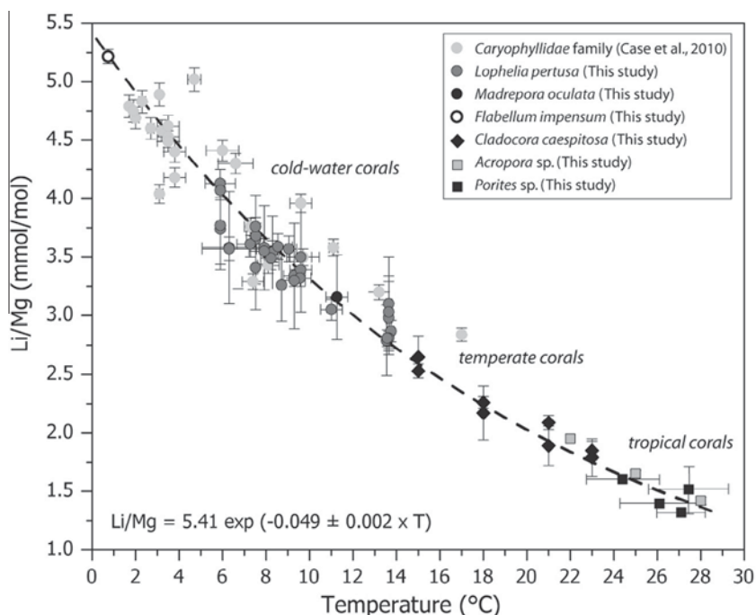
Fig. 6. Laser ablation and solution ICP-QMS Li/Mg ratios versus temperature for all specimens of cold-water, temperate and tropical corals investigated in the present study. For the laser ablation data, only the Li/Mg values specific to FA_{eq} were considered. Data from Case et al. (2010) are also reported (grey circles). The Li/Mg ratios show a strong correlation to temperature ( r^2 = 0.975 ) following an exponential regression with Li/Mg decreasing by \sim 5\% per ^{\circ}C .
