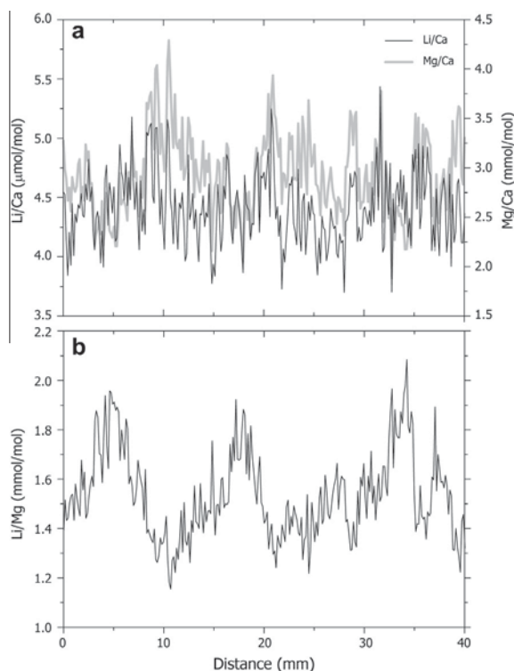
Fig. 4. Li/Ca, Mg/Ca and Li/Mg ratios obtained by laser ablation ICP-MS following a 4 cm transect along the growth axis of a Porites sp. specimen live-collected from Myrmidon Reef. Li/Ca and Mg/Ca ratios show a positive correlation, which is stronger during the summer periods compared to the winter periods. The Mg/Ca ratios exhibit a seasonal cycle with higher values during summer in accordance to results obtained from other studies on tropical corals (e.g. Mitsuguchi et al., 1996; Fallon et al., 2003). The resulting Li/Mg shows a clear seasonal cycle with lower values corresponding to the summer and vice versa.
