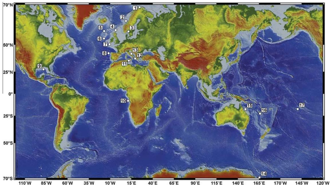
Fig. 1. Map with the locations of the coral samples analysed. 1 – Stjærnsund (POS-325-433-1; POS-325-433-2; JR-111), 2 – Sula Ridge (POS-228-216; POS-228-217; VH-95-163), 3 – Oslo Fjord (ALK-232-1050 BG), 4 – Darwin Mounds (DW1383#1), 5 – NW Rockall Bank, (POS-292-525; POS-292-526-1), 6 – SE Rockall Bank (MD01-2454G; POS-292-544-1), 7 – Porcupine Seabight (MD01-2463G; M61/3-634; POS-265-499), 8 – Galicia Bank (VH-97-351; VH-97-315), 9 – Gulf of Mexico (GoM), 10 – N'Zeta off Angola (N'Zeta), 11 – Urania Bank (M70/1-677), 12 – Apulian Bank (M70/1-721-red; M70/1-721-white; COR2-111; COR2-111(bis); COR2-84), 13 – Bari Canyon (M70/1-Dive111), 14 – Balleny Island (Fbal), 15 – Myrmidon Reef, 16 – New Caledonia (NC_2001-2004), 17 – Tahiti, Moorea (CS MOOO3A-102).
