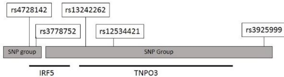
Figure 3. SNP locations in reference to the IRF5 and TNPO3 genes. The black bars show the gene locations, and the two gray boxes are two groups of SNPs that are in high linkage within the gray region, but display little association with the other SNP group. The relative locations of SNPs connected to SLE symptoms are shown.
