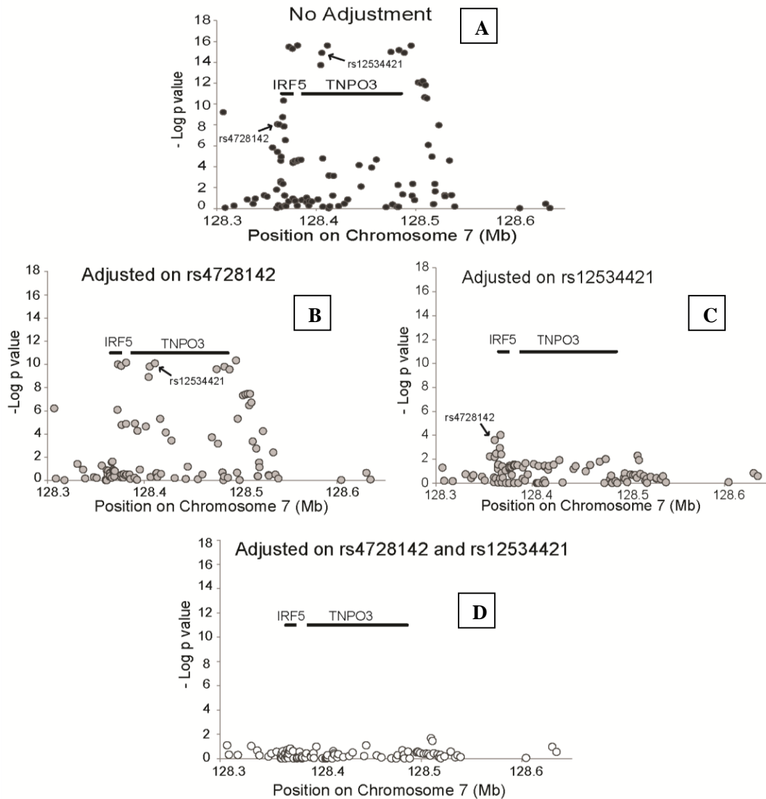
Figure 4. Conditional analysis of age-of-onset phenotype. The horizontal bars show the position on chromosome 7 of IRF5 and TNPO3 . The most associated SNPs are identified in A, B, and C. Graph A shows the statistical significance ( -\log_{10}[p\text{-value}] ) of each SNP in the IRF5/TNPO3 region. For graphs B and C, we removed each of the top two most associated SNPs. Graph D removes the association of both SNPs. From this, we conclude that rs12534421 (the second group of linked SNPs) is responsible for most of the statistical association between genetic variants and the age of onset of lupus. When the contribution of both SNPs is removed, no association remains p < 0.01 (D).
