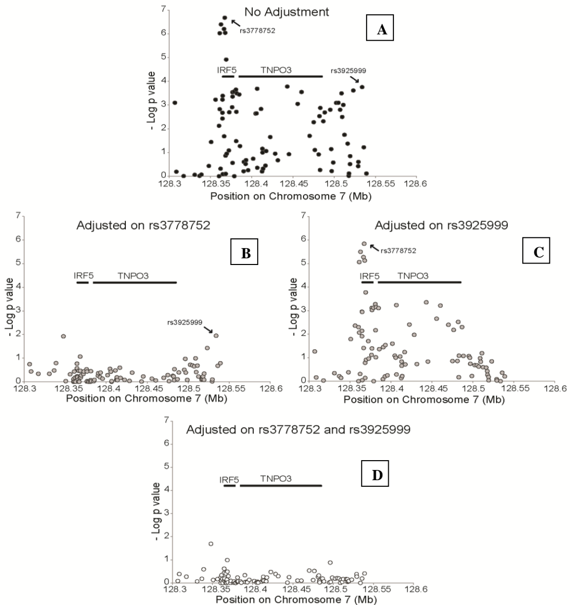
Figure 5. Conditional analysis of the presence of anti-Ro antibodies. Graph A shows the statistical significance ( -\log_{10}[\text{p-value}] ) of the association of each SNP in the IRF5/TNPO3 region with the presence of anti-Ro antibodies. For graphs B and C, we removed the association of the two most significant SNPs (which did not include rs4728142 or rs12534421) separately. The bottom graph removes the association of both SNPs. From this, we can conclude that rs3778752 (the first SNP group) is responsible for most of the statistical association of genetic variants with the presence of anti-Ro antibodies.
