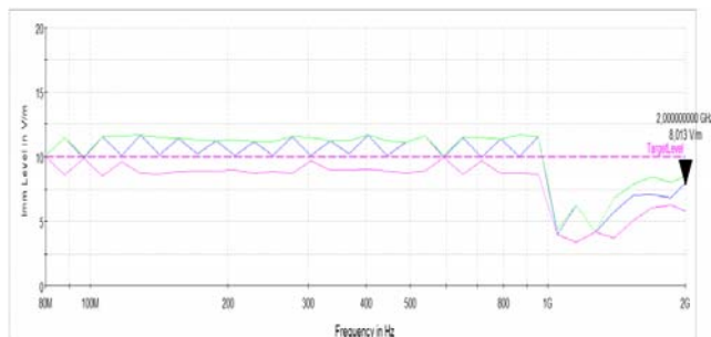
Fig. 7. Immunity level – test 2.
