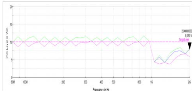
Fig. 5. Immunity level – test 1.
