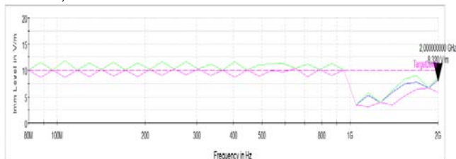
Fig. 9. Immunity level – test 3.
