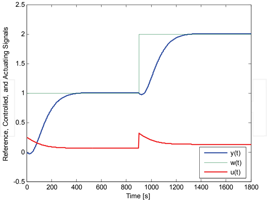
Fig. 6. Control of plant using continuous-time controller – simulation
