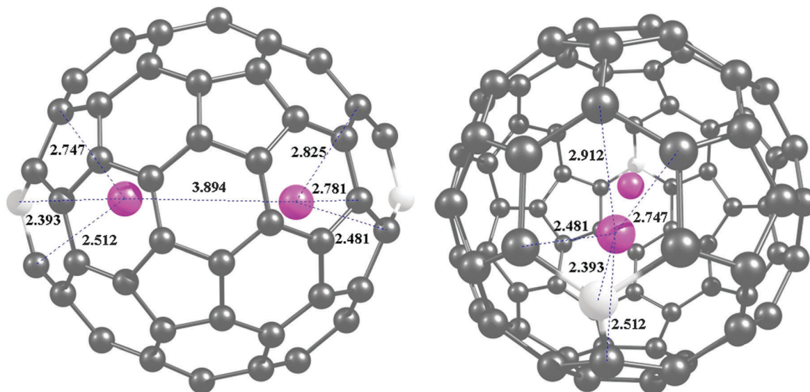
Fig. 1 The {}^7\text{U}_2@C_{80}:7 minimum structure calculated at the BP86/SVP/SDD level.
