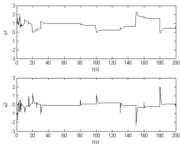
Fig. 7 Adaptive control with continuous-time controller-manipulated variables
