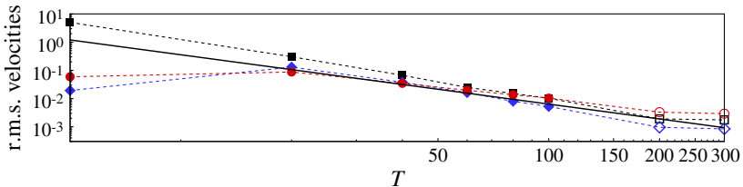
FIGURE 9. (Colour online) Root mean square values of the streamwise, wall-normal, and spanwise components of velocity (squares, u_{rms} ; diamonds, v_{rms} ; circles, w_{rms} ) versus target time, for the minimal perturbations computed for T \leq 100 and for two NLOPs. The solid line is the T^{-1.75} line passing through 1 at T=5 .
