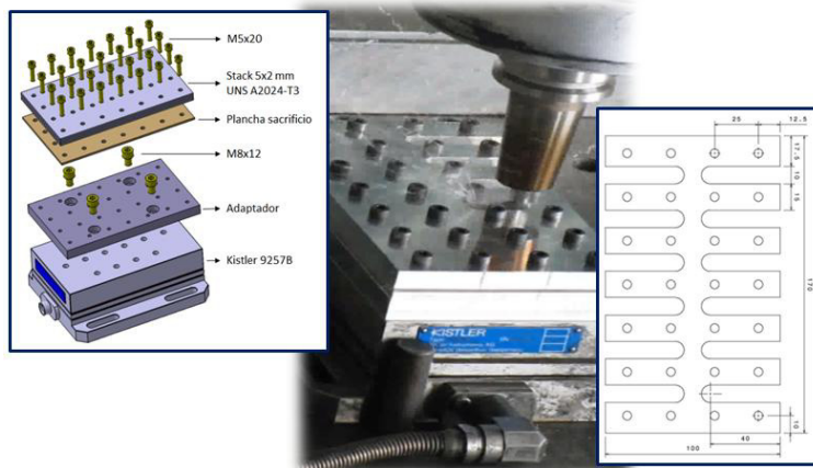
Fig. 2. Some details of the experimental configuration
