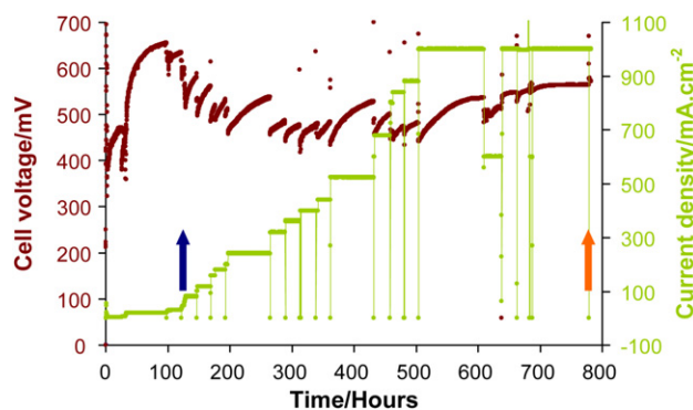
Fig. 9. Evolution of cell voltage and current density during fuel cell operation obtain with a MEA made with an ex situ aged Nafion® 212-CS membrane at 80 °C and RH = 95% during 258 days. 60 °C, 1.5 absolute bars, dry H 2 at the anode, fully humidified reactant at the cathode: O 2 except from 600 to 640 h and above 805 h where air has been used. The blue and orange arrows pointed out when the initial and final EIS measurements at 20\text{ mA cm}^{-2} with O 2 have been conducted. (For interpretation of the references to color in this figure legend, the reader is referred to the web version of the article.)
