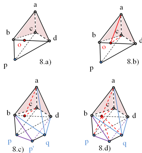
Figure 8. Example of tetrahedron split for a particularly critical interface configuration (a), its split version (b), its original adjacent tetrahedrons (c) and the updated adjacent tetrahedrons
