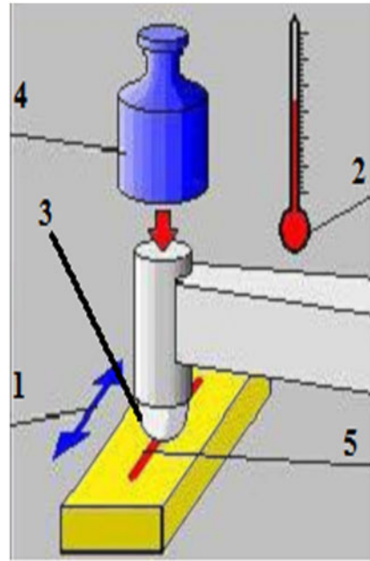
3 a photograph and b scheme of contact geometry (alternative movement) and tribotester system at CER Arts & Métiers Paris Tech ENSAM Lille [1: table, carry sample on alternative movement (wear track radius=10 mm; 2: sensor to measure heat and humidity; 3: ball 100C6 steel; 4: load applied FN; 5: sample]
