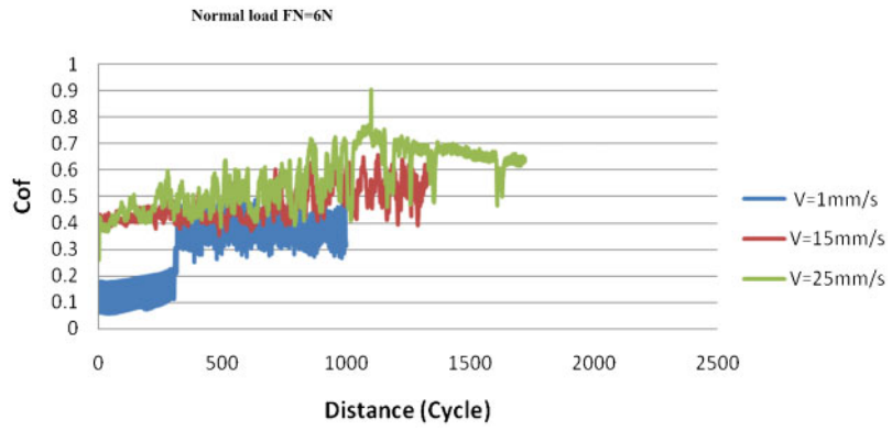
19 Friction test result of AISI 316l SS under normal load FN=6\text{ N}
