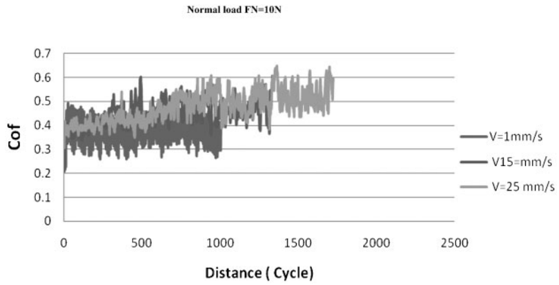
20 Friction test result of AISI 316l SS under normal load FN=10\text{ N}
