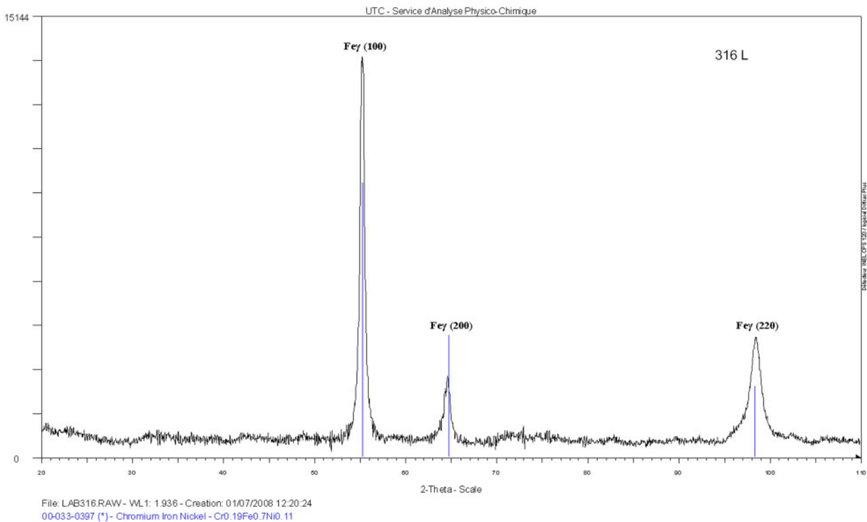
8 X-ray diffractometry spectrum of SS AISI 316L
