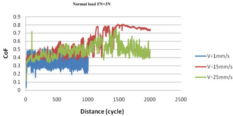
18 Friction test result of AISI 316I SS under normal load FN=3 \text{ N}
