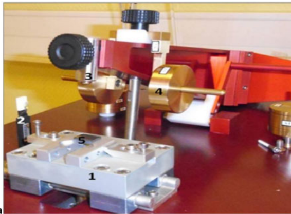
3 a photograph and b scheme of contact geometry (alternative movement) and tribotester system at CER Arts & Métiers Paris Tech ENSAM Lille [1: table, carry sample on alternative movement (wear track radius=10 mm; 2: sensor to measure heat and humidity; 3: ball 100C6 steel; 4: load applied FN; 5: sample]
