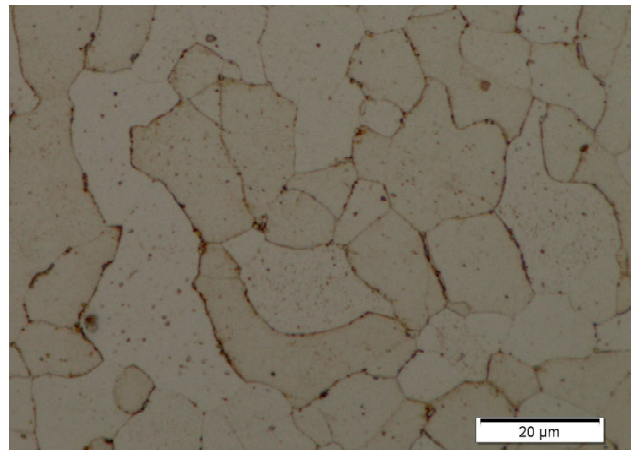
Fig. 5 (a) Microstructure of the top of laser beam formed material showing elongated ferrite and pearlite grains
