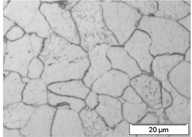
Fig. 4 Microstructure of the as received material showing equiaxed ferrite grains and pearlite
