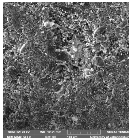
Fig. 4 SEM micrograph of Co-Cu working electrode
