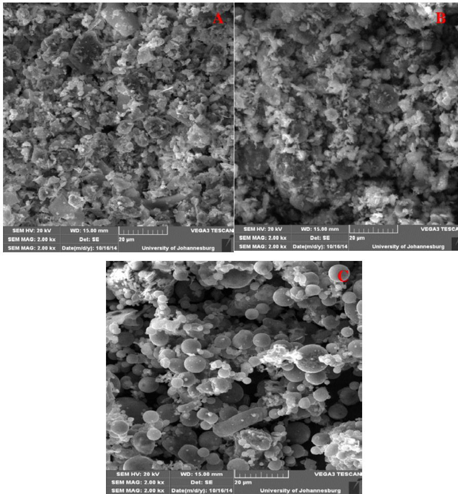
Fig.2. Showing Jarosite (A), Clay (B) and Fly ash (C) SEM microstructures
