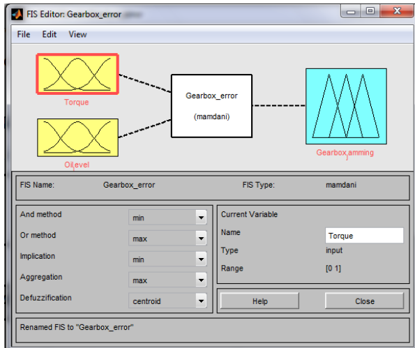
Fig 6: FIS editor for the gearbox jamming
