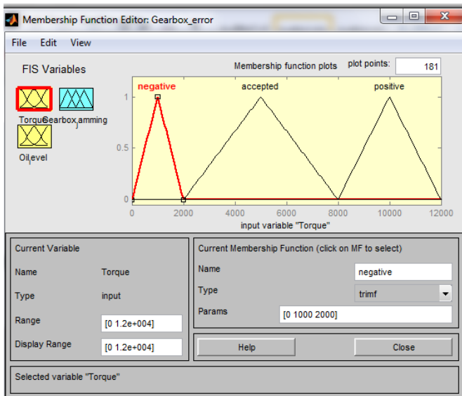
Fig 8: Membership function editor for torque monitoring
