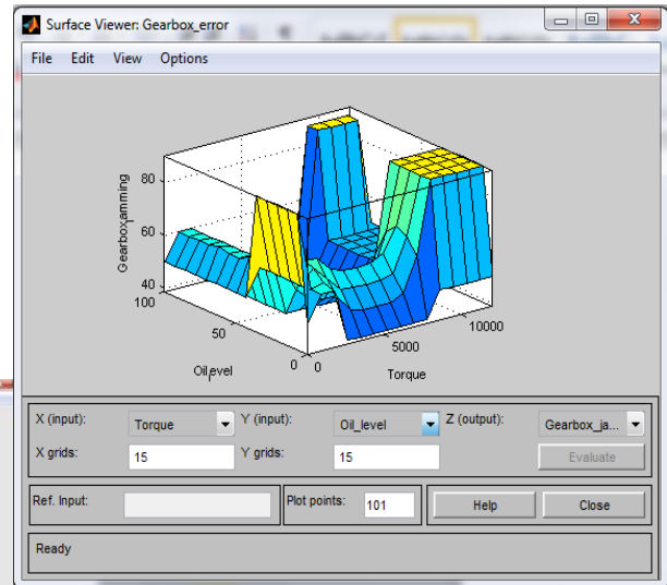
Fig 12b: Surface viewer for the gearbox monitoring
