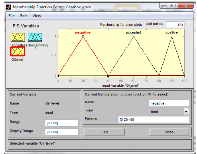
Fig 7: Membership function editor for oil monitoring
