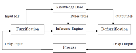
Fig 2: Fuzzy logic Control
