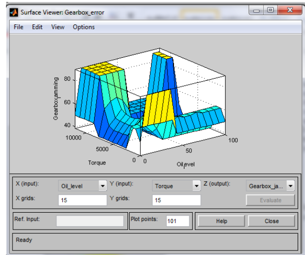
Fig 12a: Surface viewer for the gearbox monitoring showing right to left
