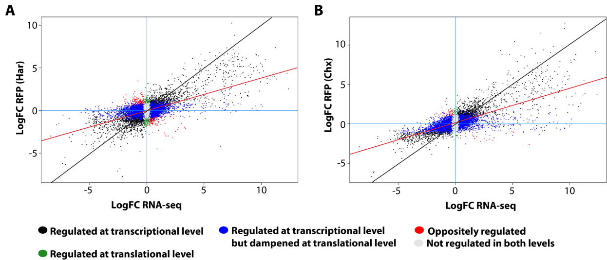
Figure 3. Changes in transcription and translation during myogenesis. Scatterplot showing differences in total RNA (x-axis) and ribosome-associated RNA (y-axis) from harringtonin (A) or cycloheximide (B) treated myoblasts and myotubes. Each data point represents the log-transformed fold change between myotubes and myoblasts. The red line indicates the slope, whereas the black line indicates the diagonal.
