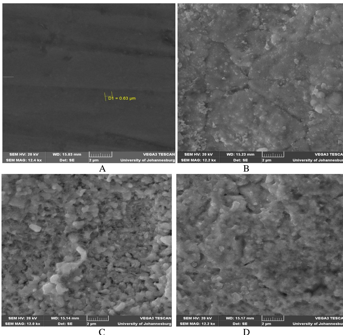
Figure 4. SEM images of (a) control sample (b) sample heat treated at 800°C (c) sample heat treated at 850°C (d) sample heat treated at 900°C before immersion in apple juice.
