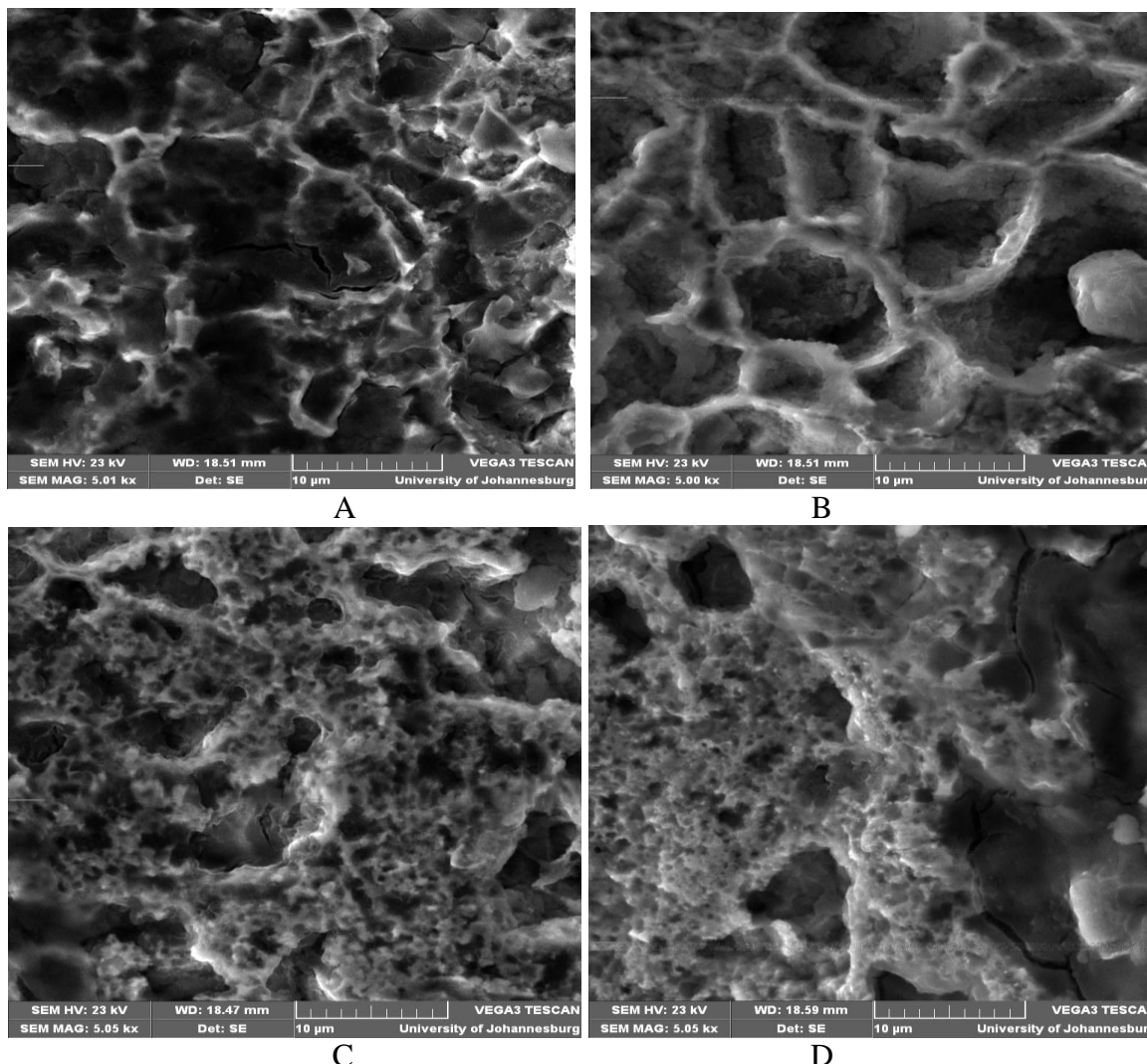
Figure 5. SEM images of (a) control sample (b) sample heat treated at 800°C (c) sample heat treated at 850°C (d) sample heat treated at 900°C after of immersion in apple juice.
