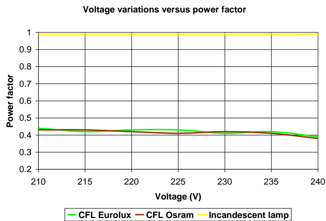
Figure 2: Effect of voltage variations on power factor for incandescent/CFLs
