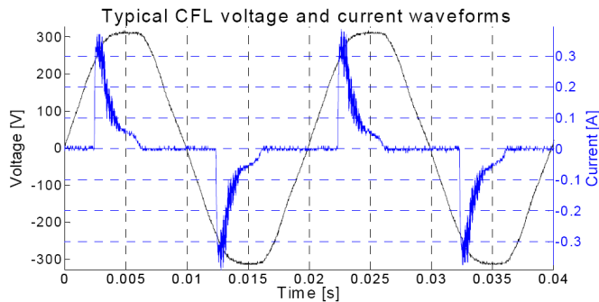
Figure 1: CFL Voltage and Current Waveforms
