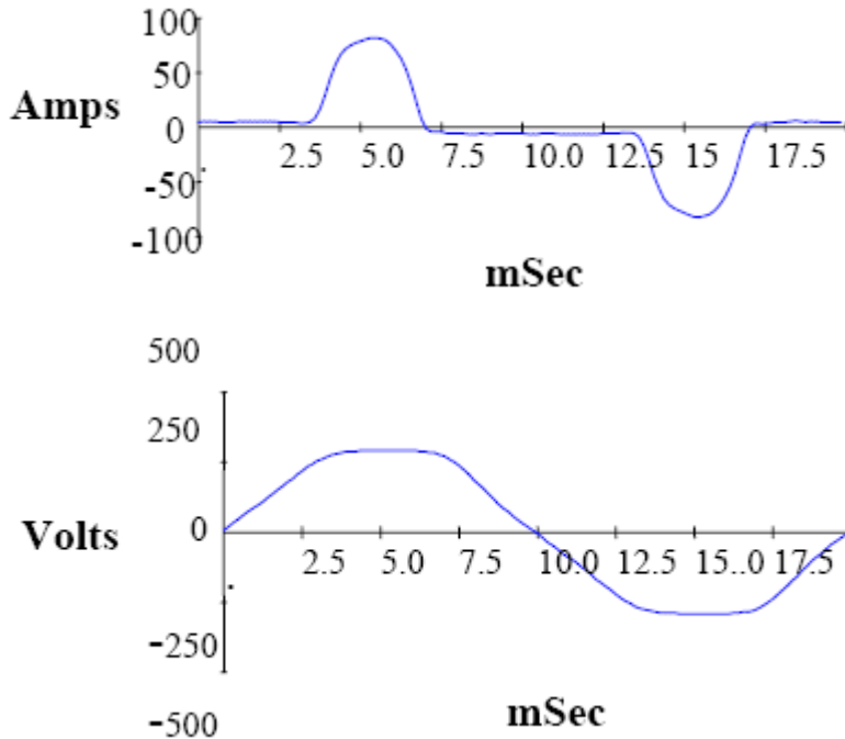
Figure 8: Current and Voltage Waveforms- Blue-phase
