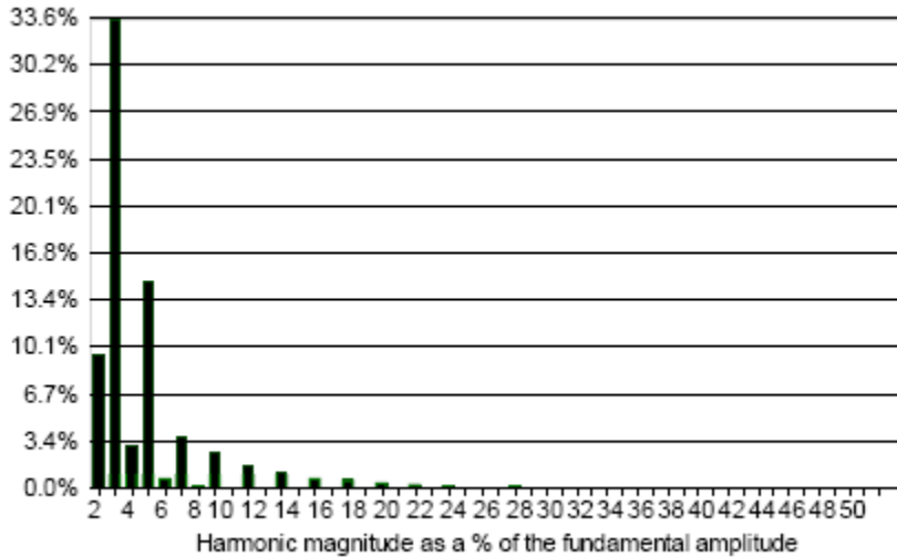
Figure 7: Microwave Current Waveform and Harmonics
