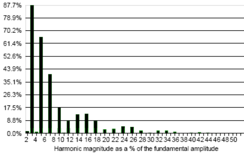
Figure 3: Personal Computer Current Waveform and Harmonics
