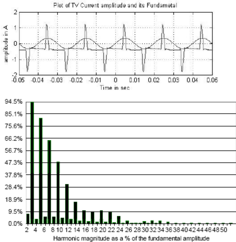
Figure 5: TV Current Waveform and Harmonic content
