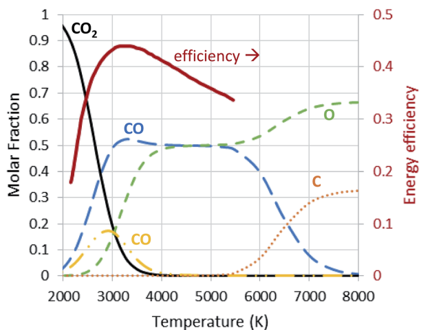
Fig. 9 Chemical equilibrium calculated molar fraction of the products of CO 2 dissociation at a fixed pressure of 100 mbar. Calculated energy efficiencies assuming instantaneous quenching after Polak et al. are plotted on the right axis.
