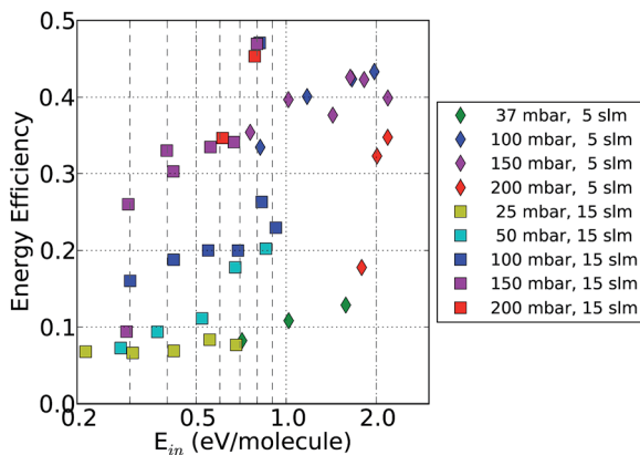
Fig. 5 Energy efficiency measured in pure microwave CO 2 plasma as a function of the specific energy input, at 5 and 15 slm gas flow rates, in scans of the reactor pressure. The underlying experimental data are identical to those of Fig. 4.
