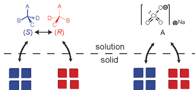
Fig. 6 Solution-solid equilibria of a chiral molecule (left) and sodium chlorate (right).
