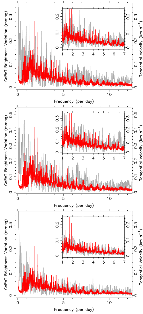
Fig. 2.— Measured amplitude spectra (grey) overlotted with the predictions of IGW for case D11 (red) for HD 46150 (top), HD 46223 (middle), and HD 46966 (bottom). The ratios between brightness and tangential velocity variations used are 2, 3, and 1.5, from top to bottom.
