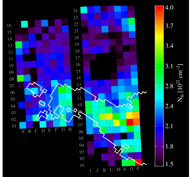
FIG. 7.— Distribution of photo-electric absorption column N_{\text{H}} derived from the spectral fits shown in Fig. 6. A clear excess of absorption is found in the lower half of the image. Over-plotted is the 15 \text{ K km s}^{-1} contour of the -33.6 to -29.6 \text{ km s}^{-1} ^{12}\text{CO} image shown in Fig. 19.
