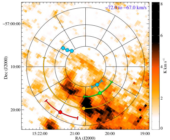
FIG. 17.— Adaptively smoothed Mopra ^{12}\text{CO} image of component 2\text{CO}_{\text{b}} in the velocity range -72\text{ km s}^{-1} to -67\text{ km s}^{-1} , same nomenclature as in Fig. 15. The CO intensity peak matches the centroid of X-ray ring [c] (yellow arc).
