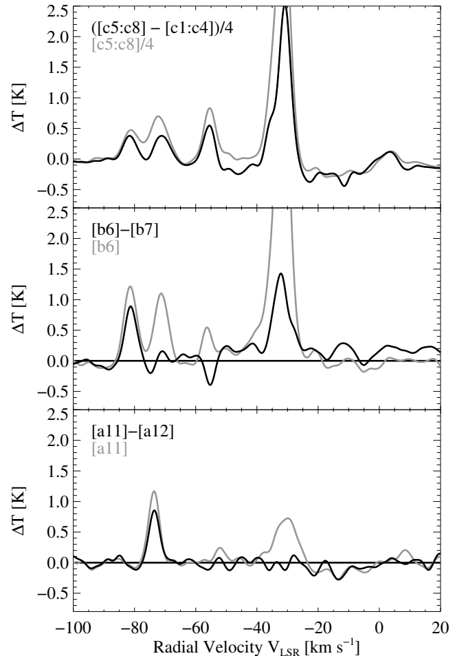
FIG. 14.— Differential (black) and total (gray) Mopra ^{12}\text{CO} spectra of three ring sections (see Fig. 8 for a definition of the ring sections), smoothed with a 3 \text{ km s}^{-1} FWHM Gaussian. Differential spectra show comparisons between neighboring ring sections that have large vs. small dust scattering intensity to isolate the CO velocity component responsible for the X-ray peak. Bottom : ring section [a11] minus [a12], middle : ring section [b6] minus [b7]; top : sum of ring sections [c5:8] minus sum of [c1:4].
