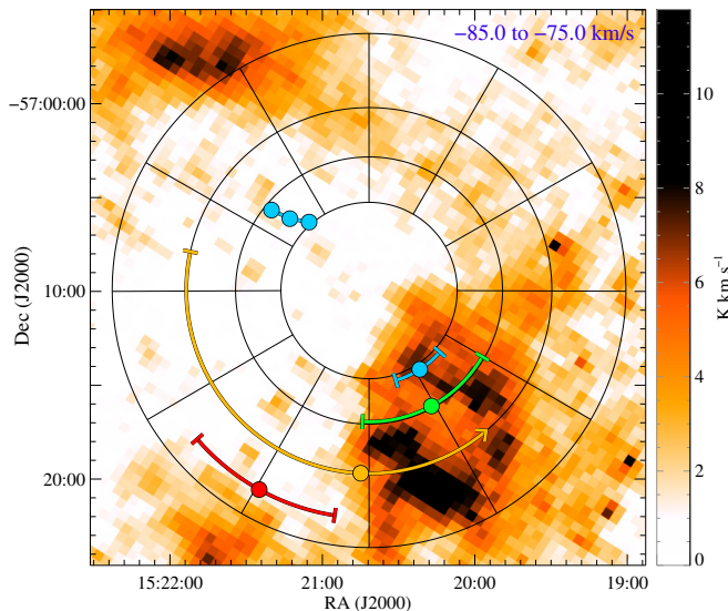
FIG. 16.— Adaptively smoothed Mopra ^{12}\text{CO} image of component 1\text{CO} in the velocity range -85\text{ km s}^{-1} to -75\text{ km s}^{-1} , same nomenclature as in Fig. 15. The CO emission in this band shows a clear peak at locations [b5] and [b6], matching the intensity distribution of X-ray ring [b] (green ring segment).
