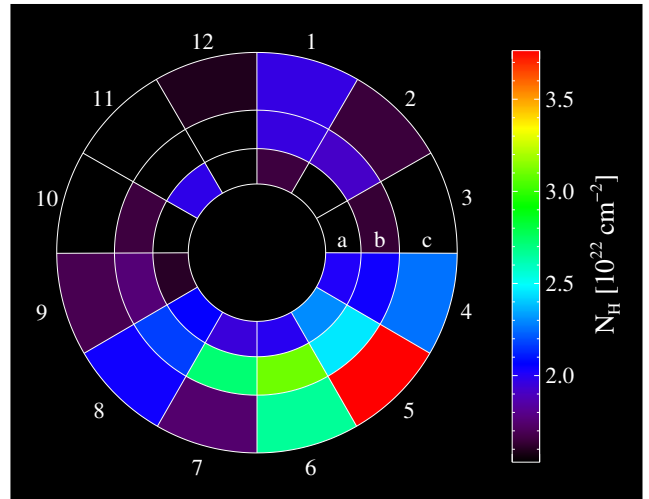
FIG. 9.— Distribution of photo-electric absorption column N_{\text{H}} derived from the spectral fits shown in Fig. 8. A clear excess of absorption is found in the lower half of the image, with a peak at position [c5].
