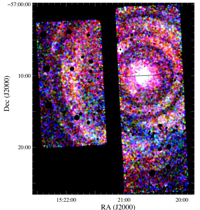
FIG. 4.— Exposure-corrected image of Chandra ObsID 15801, smoothed with a \text{FWHM} = 10.5'' Gaussian. Red: 1-2 keV, green: 2-3 keV, blue: 3-5 keV. Point sources and the read streak produced by Circinus X-1 were removed. Four separate rings of dust scattering echoes are visible in this image.
