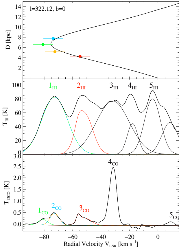
FIG. 13.— Top panel : Radial velocity as a function of distance from the Sun for the sight-line in the direction of Circinus X-1 at Galactic coordinates l = 322.12^\circ, b = 0^\circ , using the rotation curves from McClure-Griffiths & Dickey (2007) and Brand & Blitz (1993) for the inner and outer Galaxy, respectively. Overplotted are the locations and radial velocities for the four dust clouds [a]-[d] (from top to bottom) responsible for the dust scattering rings, assuming the best fit distance of 9.4 kpc. Middle panel : 21cm HI spectrum integrated over rings [a]-[c] defined in Fig.8. Component 1_{\text{HI}} comprises CO components 1_{\text{CO}} and 2_{\text{CO}} listed below. Bottom panel : ^{12}\text{CO} spectrum integrated over the same region of rings [a]-[c] from Fig. 8, smoothed with a 2 \text{ km s}^{-1} FWHM Gaussian. Five discernible velocity components are labeled 1_{\text{CO}}-5_{\text{CO}} .
