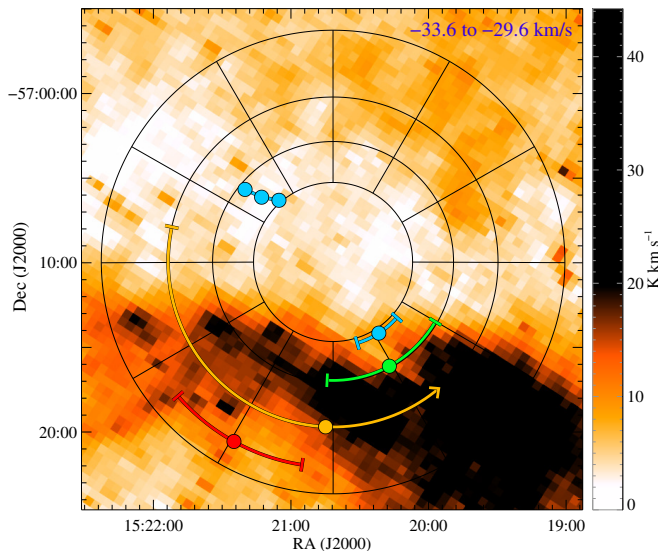
FIG. 19.— Adaptively smoothed Mopra ^{12}\text{CO} image of component 4\text{CO} in the velocity range -33.6\text{ km s}^{-1} to -29.6\text{ km s}^{-1} , showing the brightest emission feature in the field of view; same nomenclature as in Fig. 15. The band of molecular gas across the lower half of the image matches the band of absorption seen in the color images in Fig. 4 and 5 in position and morphology and corresponds to the excess absorption found in the spectrally determined absorption column shown in Figs. 7 and 9.
