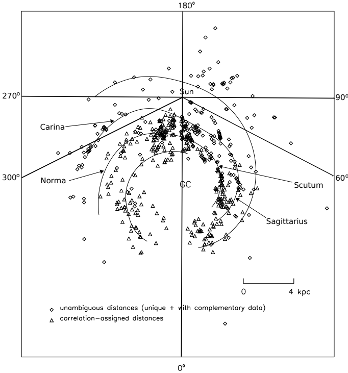
Fig. 3. The distribution of star-forming regions (H II regions) in the inner Galaxy, from Paladini et al. (2004) Fig. 12, with the l = 300^\circ \rightarrow 0^\circ \rightarrow 60^\circ sector indicated. The relevant spiral arms are also indicated.
