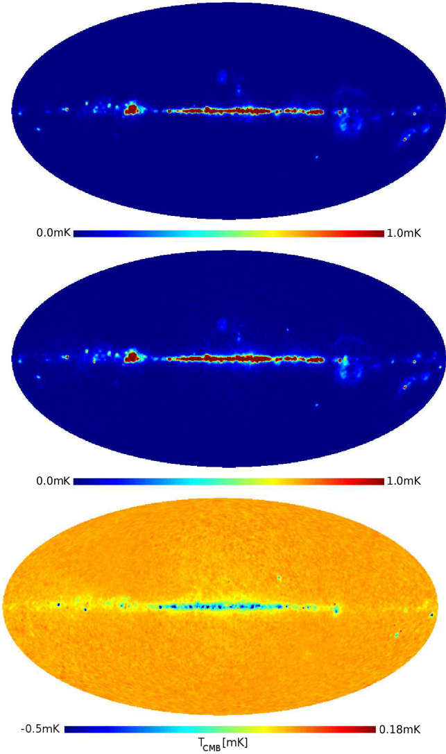
Fig. A.2. The input, reconstructed and residual maps of the free-free emission at 70.4 GHz. All maps are in Mollweide projection, smoothed with a 1^\circ beam, N_{\text{side}} = 128 . The colour scale is linear, and the units are \text{mK}_{\text{CMB}} .
