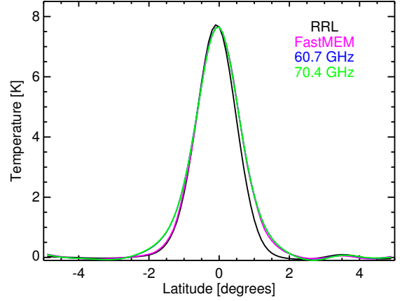
Fig. 6. Latitude cuts for the narrow free-free-related component in the longitude range l = 20^\circ to 30^\circ for RRLs, FastMEM, WMAP 60.7 GHz, and Planck 70.4 GHz. These are normalized to match the FastMEM solution at b = 0^\circ in order to show their relative widths. The re-scaled 60.7 GHz and 70.4 GHz cuts match at all latitudes and are thus not visible separately.
