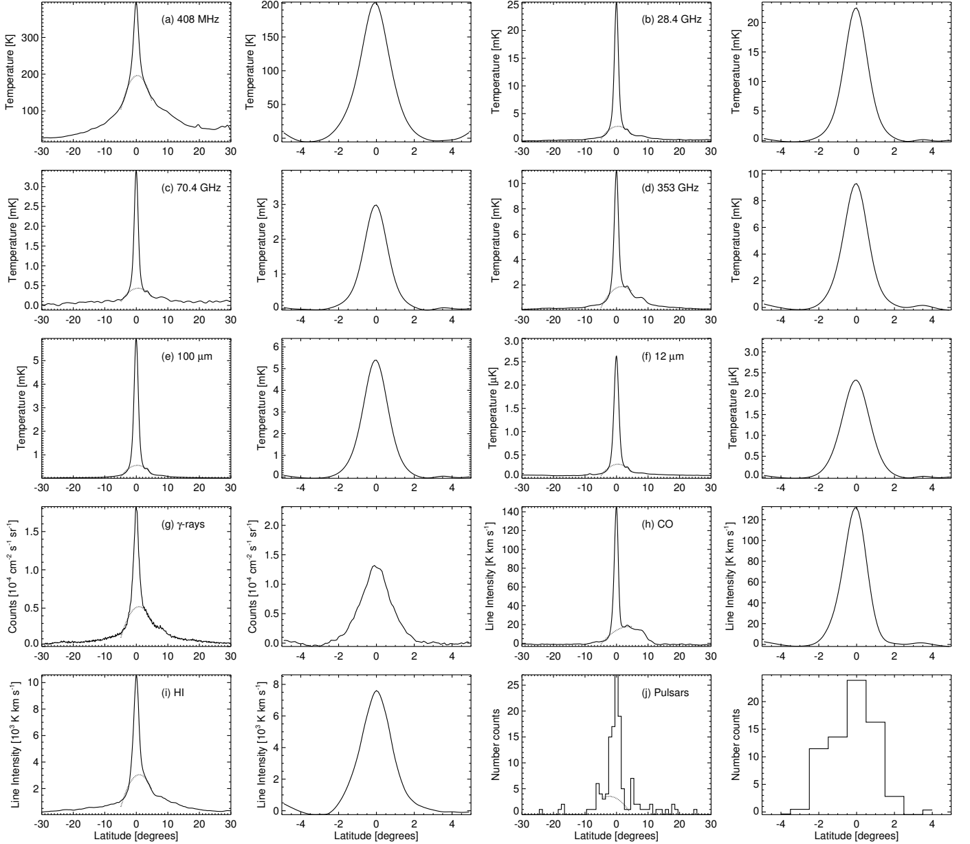
Fig. 4. Latitude distribution of various components averaged over the longitude range 20^\circ to 30^\circ . The first and third columns show the total emission ( solid line ) with the parabolic fit ( dotted line ) and the second and fourth columns show the narrow component. The pulsar data are at N_{\text{side}} = 64 to account for the low sampling and include all ages; young and old pulsars are shown separately in Fig. 7. The northern Gould Belt system can be seen at positive latitudes at all frequencies. The broad 15^\circ wide synchrotron component is evident in the 408 MHz cut.
