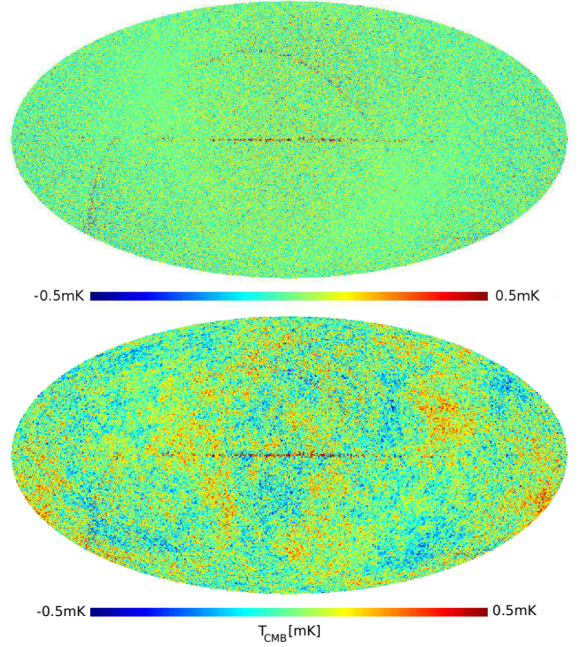
Fig. A.1. Simulated data: residual maps at 70.4 GHz, containing only receiver noise and point sources (Eq A.1, upper panel) and CMB component-cleaned map (Eq A.2, lower panel). The maps are in Mollweide projection, with N_{\text{side}} = 1024 and a linear temperature scale with units of T_{\text{CMB}} .
