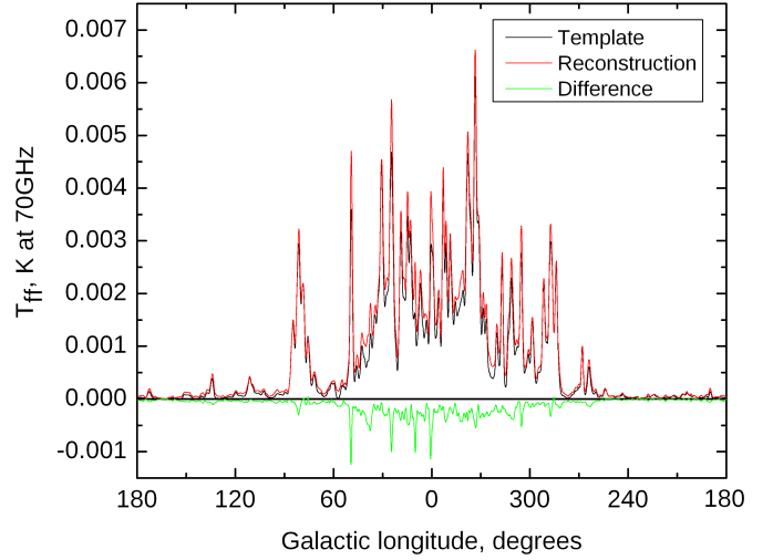
Fig. A.3. The input, reconstructed and residual Galactic plane profiles for the free-free emission at 70.4 GHz. Profiles were calculated over the maps shown in Fig. A.2; units are \text{K}_{\text{CMB}} . The plots are made for a 1^\circ -resolution cut along the Galactic plane.
