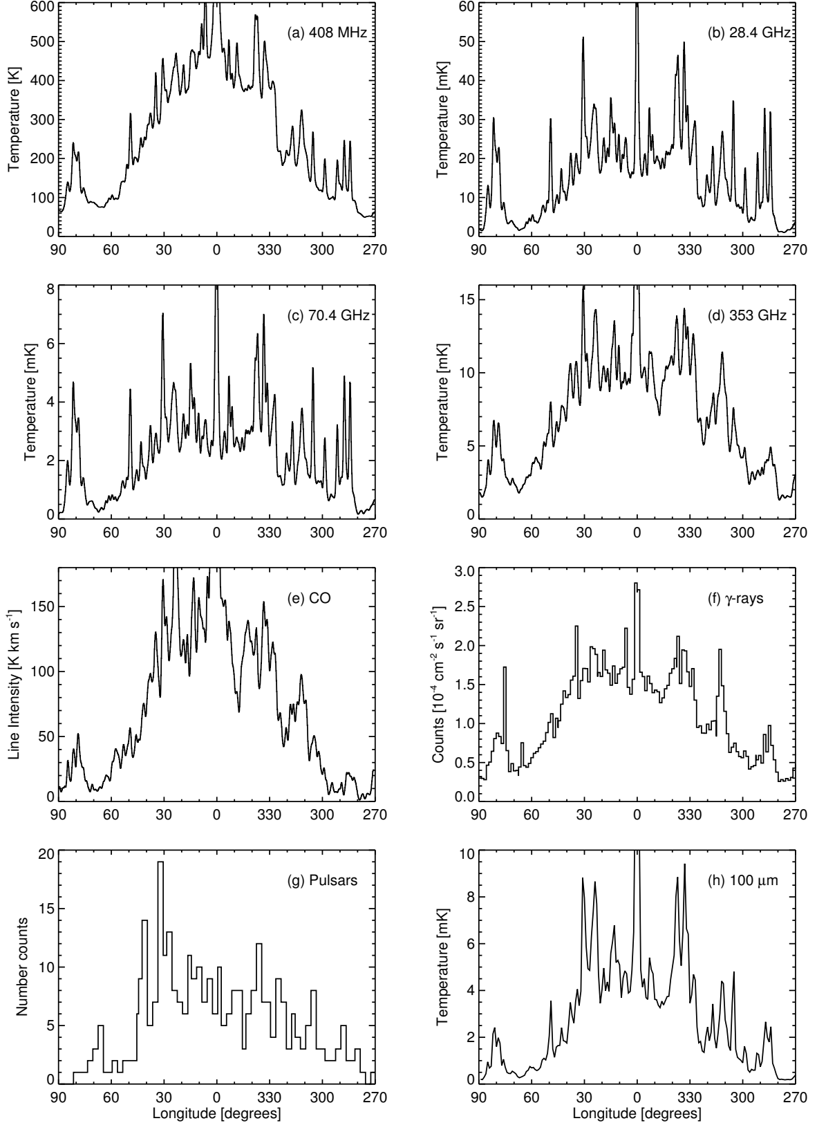
Fig. 5. The longitude distribution of emission components along the Galactic plane at b = 0^\circ in the range l = 90^\circ to 270^\circ . The data are all smoothed to 1^\circ resolution except the gamma-ray data with a FWHM of 88' . The components shown are 408 MHz (mainly synchrotron), 28.4 GHz (similar AME and free-free), 70.4 GHz (mainly free-free), 353 GHz (dust), CO, gamma-rays, pulsar numbers (representing supernovae), and 100 \mu\text{m} . The gamma-ray and pulsar data are at N_{\text{side}} = 64 and N_{\text{side}} = 32 respectively, to account for the relatively low sampling. The pulsar data are uniformly surveyed from l = 270^\circ to 40^\circ ; at l = 40^\circ to 90^\circ the survey sensitivity is lower. The Galactic centre is off-scale so that the diffuse emission can be displayed.
