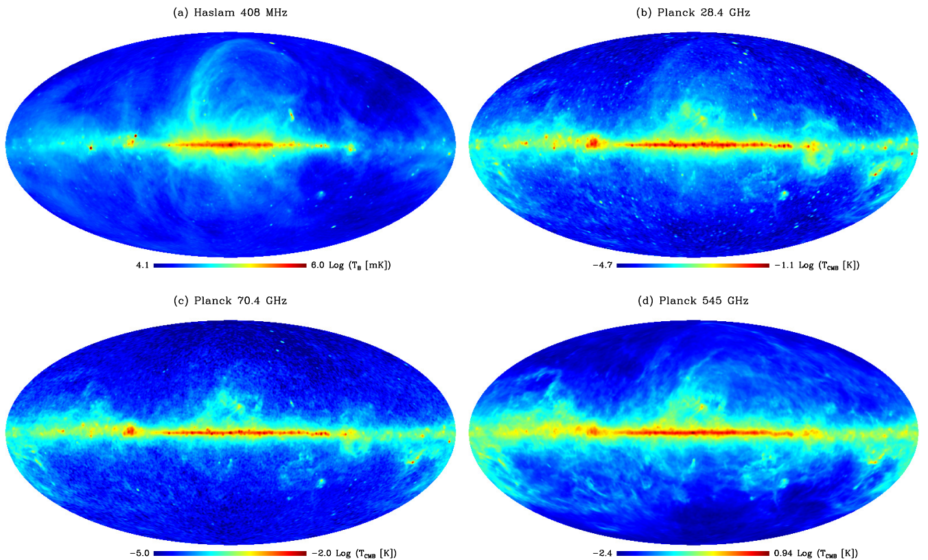
Fig. 1. The whole sky map at four frequencies showing the narrow inner Galaxy emission: (a) the 408 MHz map of Haslam et al. (1982) , (b) the 28.4 GHz map from Planck , (c) the 70.4 GHz map from Planck , and (d) the 545 GHz map from Planck . The colour scales are logarithmic, and the maps are in Mollweide projection.
