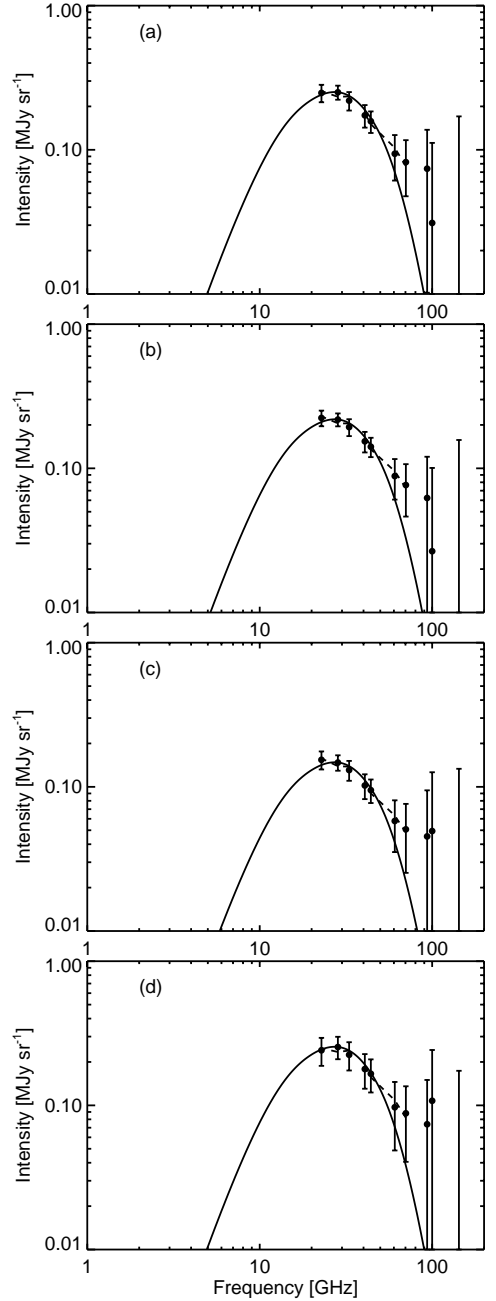
Fig. 10. AME spectra for the longitude ranges (a) l = 20^\circ\text{--}30^\circ , (b) 30^\circ\text{--}40^\circ , (c) 320^\circ\text{--}330^\circ , and (d) 330^\circ\text{--}340^\circ . The spectra cover the frequency range 23–143 GHz and are in units of intensity. The conversion factor from intensity to brightness temperature at 28.4 GHz is 40 \text{ mK MJy}^{-1} \text{ sr} .
