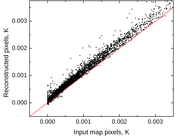
Fig. A.4. T - T plot comparing the pixel values in the simulated input map and in the reconstructed map. The solid red line indicates equality. The frequency is 70.4 GHz and the temperature scale is \text{K}_{\text{CMB}} .
