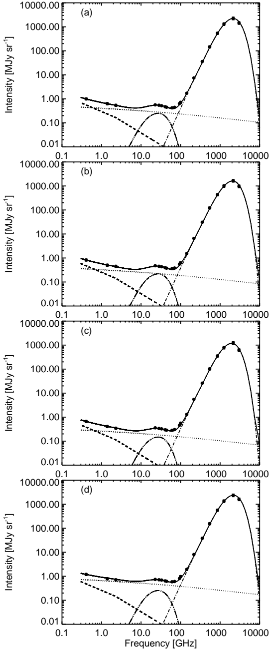
Fig. 9. SEDs over full frequency range 0.408 GHz to 3000 GHz, for the longitude ranges (a) l = 20^\circ\text{--}30^\circ , (b) 30^\circ\text{--}40^\circ , (c) 320^\circ\text{--}330^\circ , and (d) 330^\circ\text{--}340^\circ . The points show the total emission, which is separated into free-free from the RRL and FastMEM data ( dotted line ), synchrotron from the free-free-corrected 408 MHz data ( dashed line ) and thermal dust ( dot-dashed line ). The total of the four components is given by the full line. AME is the residual ( long-dash-dotted line ). The conversion factor from intensity to brightness temperature at 28.4 GHz is 40 \text{ mK MJy}^{-1} \text{ sr} .
