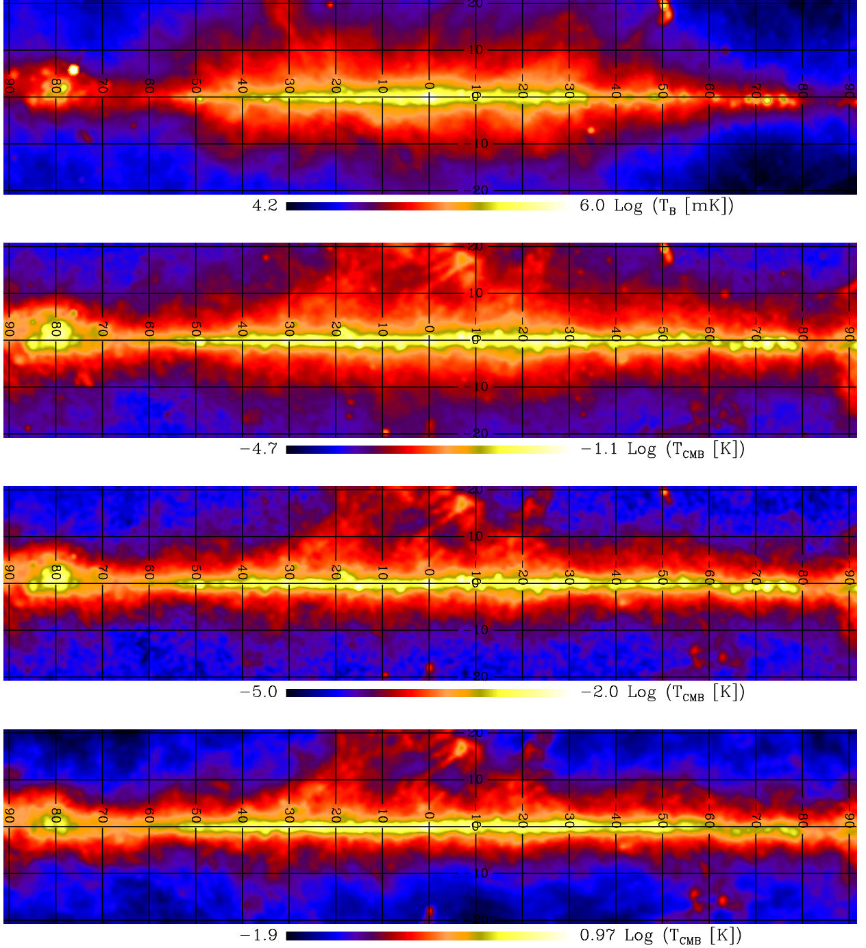
Fig. 2. The narrow Galactic emission at four frequencies: (a) the 408 MHz map of Haslam et al. (1982) , (b) the 28.4 GHz map from Planck , (c) the 70.4 GHz map from Planck , and (d) the 545 GHz map from Planck . The colour scales are logarithmic. The longitude range is l = 270^\circ \rightarrow 0^\circ \rightarrow 90^\circ ; the latitude range is -20^\circ to +20^\circ . The maps are in Cartesian projection.
