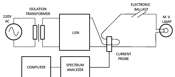
Fig. 3. Set-up for Measurements in the 3kHz – 30MHz Range (Electronic Ballast).
