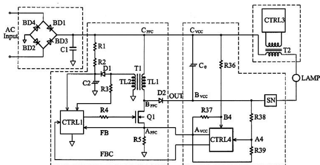
Fig. 5. Electronic ballast driver for mercury vapor lamp.
