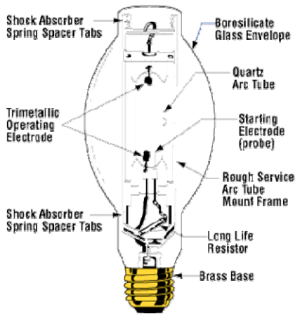
Fig. 1. The Inside Structure Of the Mercury Vapor Lamp [5].
