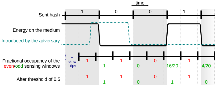
Figure 2.3: The attack found by model checking, for a 4-bit hash. The adversary introduces energy to the medium to change the received hash to 1010.
