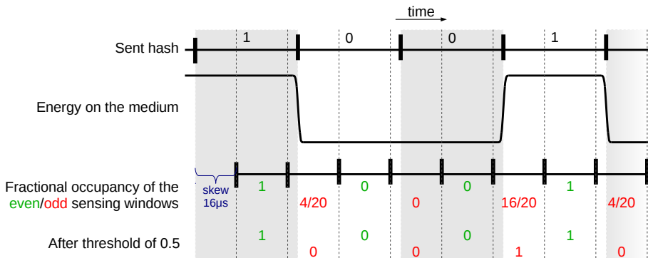
Figure 2.2: Sending and receiving the slots of a 4-bit hash. The even sensing windows have the higher variance here. Therefore, those represent the received hash. Clock skew ( 16 \mu\text{s} ) is shown in blue on the left.
