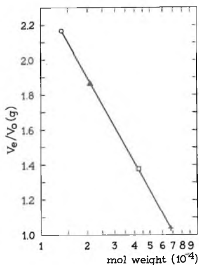
Fig. 1b. Graphical interpretation of the elution data from fig. 1a. \circ RNAase; \blacktriangle CM- \alpha_1 ; \square ovalbumin; + serum albumin.
