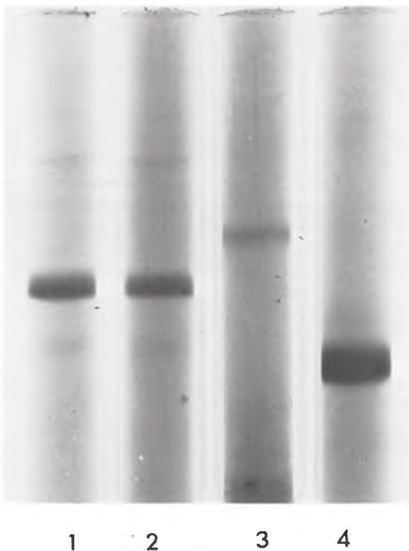
Fig. 4a. Electrophoresis on polyacrylamide-SDS gels. 1) CM- \alpha_1 incubated in 2% SDS for 17 hr at 37°; 2) CM- \alpha_1 untreated; 3) trypsin; 4) ribonuclease. The electrophoretic experiment was performed according to Shapiro et al. [15] with the modification of double cross linking of the gels.
