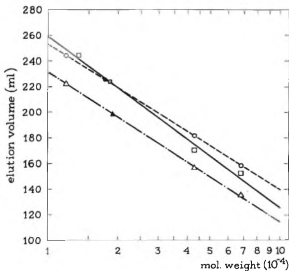
Fig. 2. Graphical interpretation of elution data of separated fractions from a Sephadex G-100 column equilibrated with 6 M urea-0.05 M phosphate buffer at pH 7.6. —○— serum albumin, ovalbumin, cytochrome c and CM- \alpha ; — \Delta — serum albumin, ovalbumin, cytochrome c and CM- \alpha 1 ; —□— serum albumin, ovalbumin, ribonuclease and CM- \alpha 2 .
