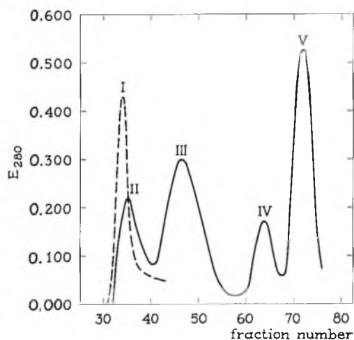
Fig. 1a. Elution profile of separated fractions from a Bio-gel A5M agarose column equilibrated with 6 M guanidine-HCl. Analysis for protein was carried out automatically on a LKB Uvicord at 280 nm. I, Blue dextran (630 nm), II, serum albumin III, ovalbumin, IV, CM- \alpha_1 , V, RNAase.
