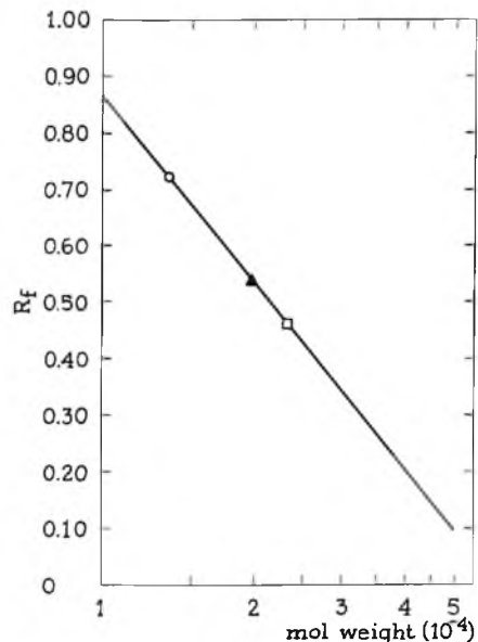
Fig. 4b. Graphical interpretation of the electrophoretic migration data of the different proteins shown in fig. 4a. \circ RNase; \blacktriangle CM- \alpha_1 ; \square trypsin.
