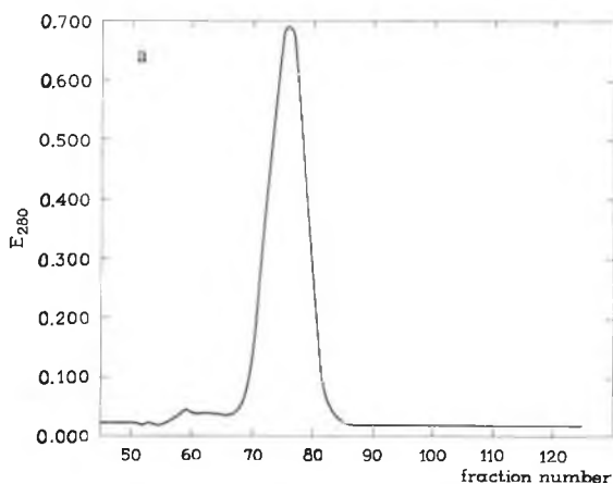
Fig. 3. Gel filtration on G-100 urea columns of CM- \alpha 2 a) after incubation in 6 M urea for 3 days mixed with untreated CM- \alpha B; b) after incubation in 6 M urea for 3 days mixed with ribonuclease.
