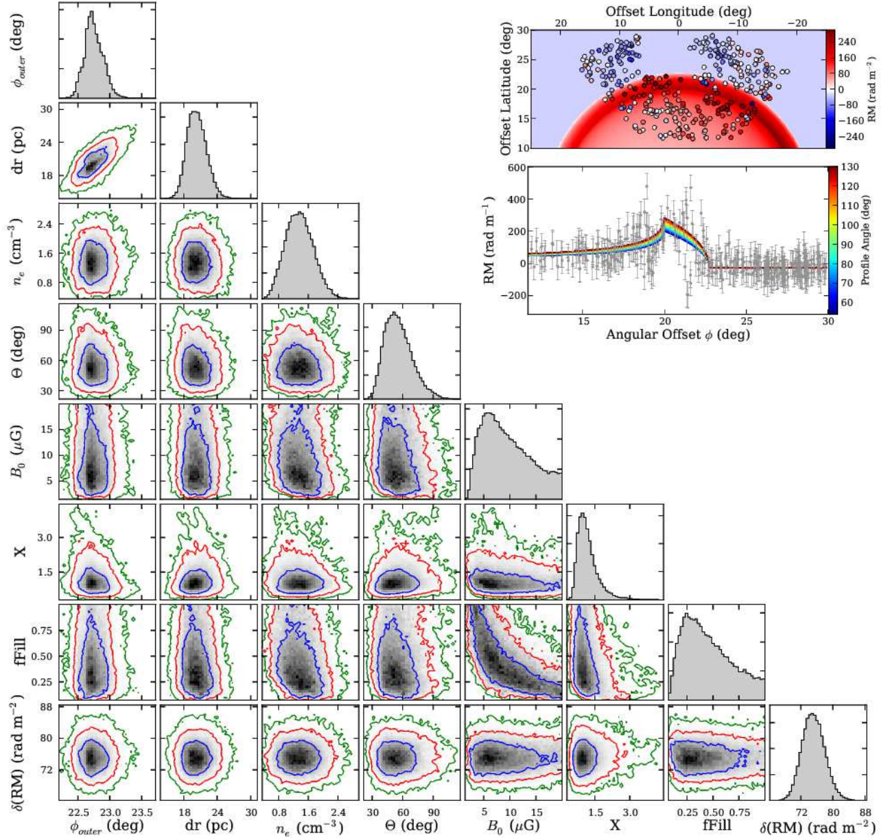
Fig. 9.— Main-figure : Triangular grid of confidence plots for the Gum Nebula, produced by fitting the ionised shell model to the Taylor et al. (2009) RM-catalogue assuming a flat background (also see Table 2). The blue, red and green contours represent the 1\sigma , 2\sigma and 3\sigma confidence intervals, respectively. The filled histograms on the diagonal show the marginalised likelihood distributions for each free parameter in the model. Inset : The rotation measure image ( top ) and azimuthal profile ( bottom ) for the best fitting model over-plotted by the selected RM data from the Taylor et al. (2009) catalogue. Note the compressed range in angular offset on the x-axis of the inset panel, compared to the equivalent plots in Fig. 7.
