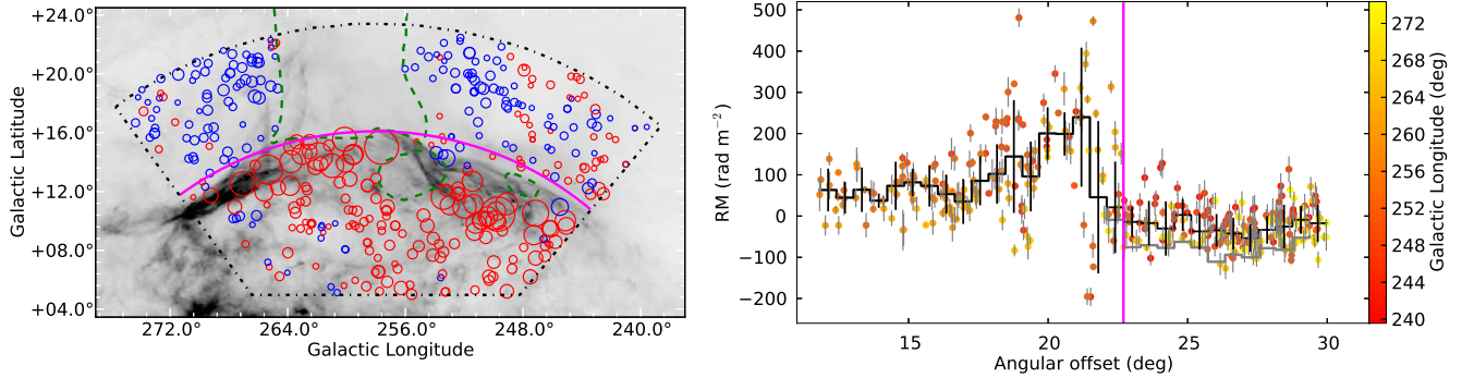
Fig. 3.— Left : Positions of polarised extragalactic sources selected for analysis from the Taylor et al. (2009) catalogue. Red and blue circles indicate positive and negative RMs, respectively, and the radius of each circle is scaled to the absolute value of the RM. The green dashed lines enclose regions where sources have been excised from the sample because they likely probe a contaminating region, or are obvious outliers ( > 3\sigma ). Right : RMs plotted as function of angular offset from the centre of the nebula. The formal uncertainties in the catalogue are represented by vertical grey lines (scaled \times 2 for clarity) and each point is colour-coded for Galactic Longitude. The solid black histogram represents a median-binned version of the plot, with bin-sizes of 0.6^\circ . The solid grey histogram illustrates the level of the RMs exterior to the nebula before the discrete object correction was applied. Vertical black error-bars illustrate the 1\sigma scatter in each bin. The magenta line in both panels indicates the outer boundary of the nebula. In both panels the RMs are plotted assuming a flat background, i.e., no correction has been made for a large-scale RM-gradient due to the Galaxy in the background (or foreground). The effect of subtracting different model backgrounds is illustrated in Fig. 4 and discussed in §2.2.1.
