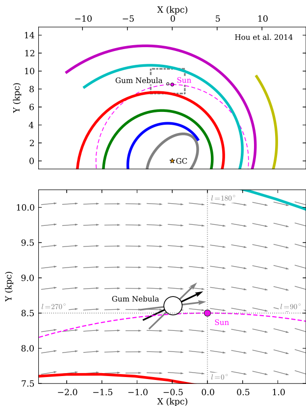
Fig. 12.— Top panel: Cartoon showing the location of the Gum Nebula in the disk of the Milky Way. The coloured lines trace the polynomial-logarithmic spiral arm models of Hou & Han (2014). A dashed magenta line plots the solar circle at a Galactic radius of 8.5 kpc. Bottom panel: Illustration of the fitted magnetic field orientation around the Gum Nebula. The plot covers the region inside the grey box in the upper panel and the Gum nebula is shown by a black circle (to scale). The three thick arrows piercing the Gum Nebula show the median (black) and \pm 1 -sigma ranges (grey) of field orientation found by fitting the RMs in §4.2. The field of thin grey vectors depicts the orientation of a spiral magnetic field with a pitch-angle of \varphi = -7.2^\circ .
