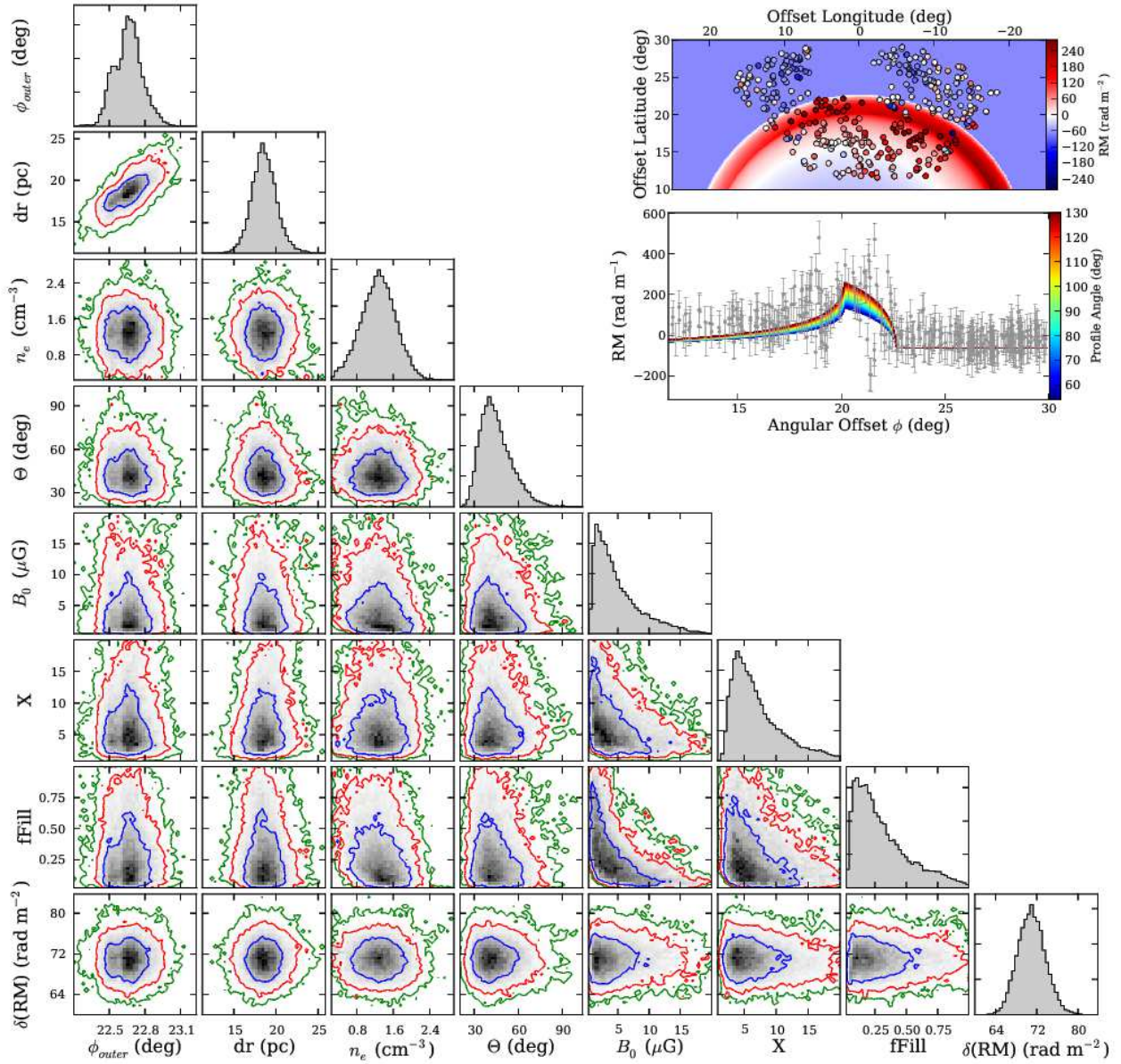
Fig. 10.— As for Fig. 9, but assuming a background as given by Sun et al. (2008).
