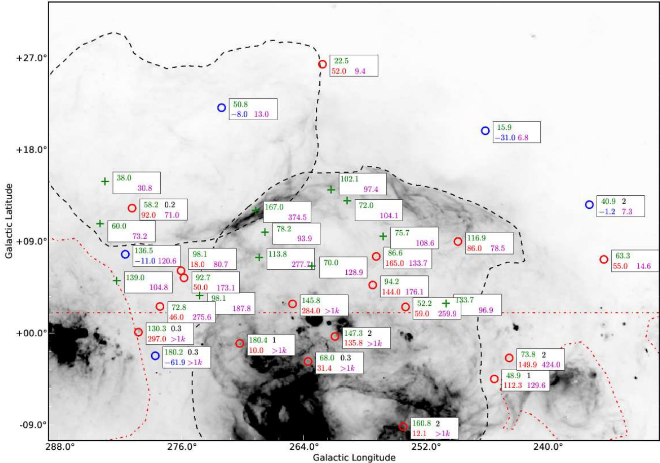
Fig. 6.— Selection of pulsars with known DM values towards the Gum Nebula. All pulsars with b > 2^\circ are shown alongside a selection of pulsars with accurate distances below b = 2^\circ . Red dot-dashed lines outline confounding parts of the Galactic plane and pulsars in these regions have been omitted. ‘o’ symbols represent pulsars with both DM and RM measurements, and ‘+’ symbols represent pulsars with only DM measurements. Each pulsar is annotated with its DM in \text{pc cm}^{-3} (top-left number, coloured green), RM in \text{rad m}^{-2} (bottom-left number, coloured red or blue signifying positive or negative RM, respectively), independently determined distance in kpc, where known (top-right number, coloured black) and EM in \text{pc cm}^{-6} (bottom-right number, coloured magenta).
