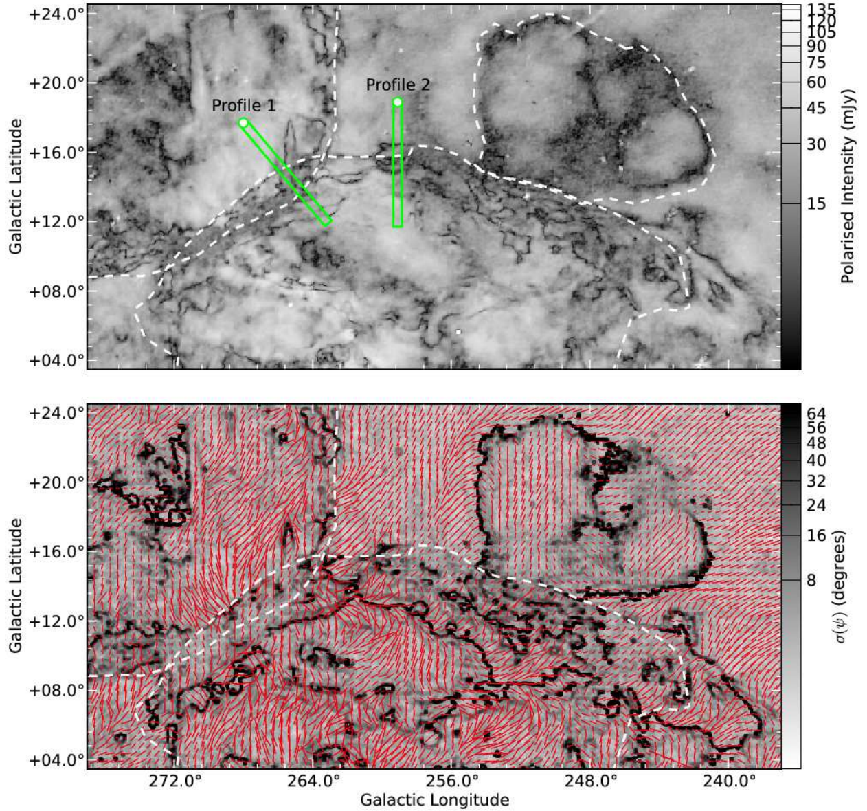
Fig. 13.— Top panel: Map of the 2.3GHz polarised intensity for the upper Gum Nebula. Green rectangles show where profiles have been extracted, in Fig. 14 and dotted lines outline the Gum Nebula and Antlia SNR. The profiles run from (l, b) = (268.0^\circ, 17.7^\circ) to (263.1^\circ, 11.9^\circ) and (259.1^\circ, 18.9^\circ) to (259.1^\circ, 11.7^\circ) for profiles 1 and 2, respectively. Bottom panel: Map of the dispersion in polarisation angle \sigma(\psi) . The value of \sigma(\psi) in each pixel has been calculated from the standard deviation within a beam-sized aperture. Dark canals correspond to regions where the polarisation angle varies by close to 90^\circ within a beam. The red bars over-plotted on the image every 7th pixel illustrate the orientation of the polarisation vectors (magnetic vector, not corrected for RM).
