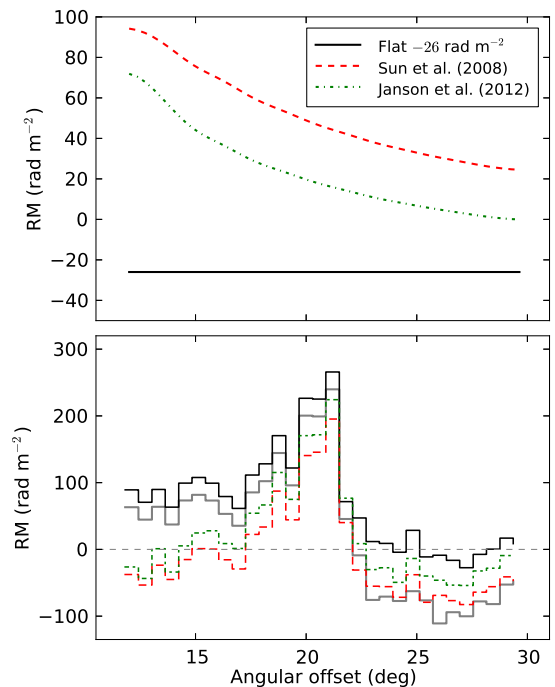
Fig. 4.— Top : Sample profiles at l = 259^\circ from the models of Sun et al. (2008) and Jansson & Farrar (2012) illustrating the predicted RM-gradient with Galactic latitude. Bottom : The light-grey histogram is the azimuthally averaged RM-profile of the Gum Nebula uncorrected for discrete contaminating sources or large-scale RM background (also plotted in Fig. 3). The black histogram is the equivalent with discrete corrections applied and a flat background of -26.4 \text{ rad m}^{-2} subtracted. The red (dashed) and green (dot-dashed) histograms illustrate the effect of subtracting the 2-D Sun et al. (2008) and Jansson & Farrar (2012) RM-models, respectively, from each point source select from the Taylor et al. (2009) catalogue. Note that the discrete corrections have previously been applied. In both cases the large-scale gradient correction acts to decrease the RMs in the interior of the nebula relative to the exterior.
