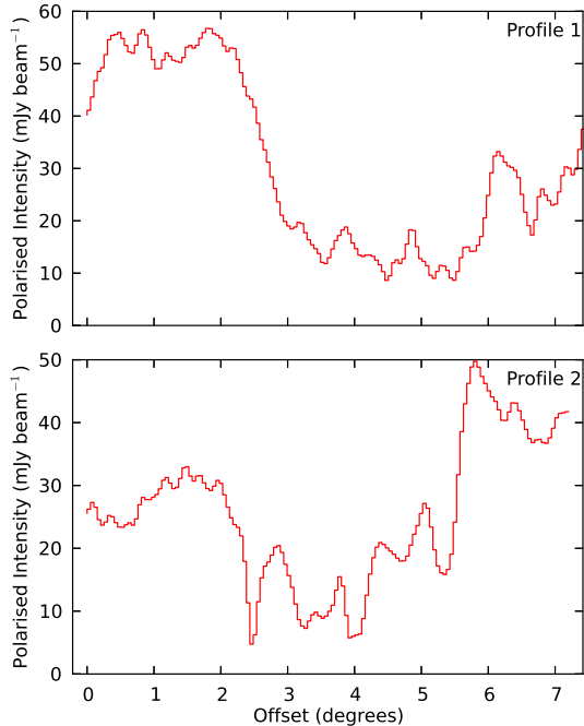
Fig. 14.— Two profiles extracted from the map of the 2.3 GHz polarised intensity. The tracks along which the profiles have been extracted are illustrated by the green boxes in Fig. 13 and the starting positions marked by circles.
