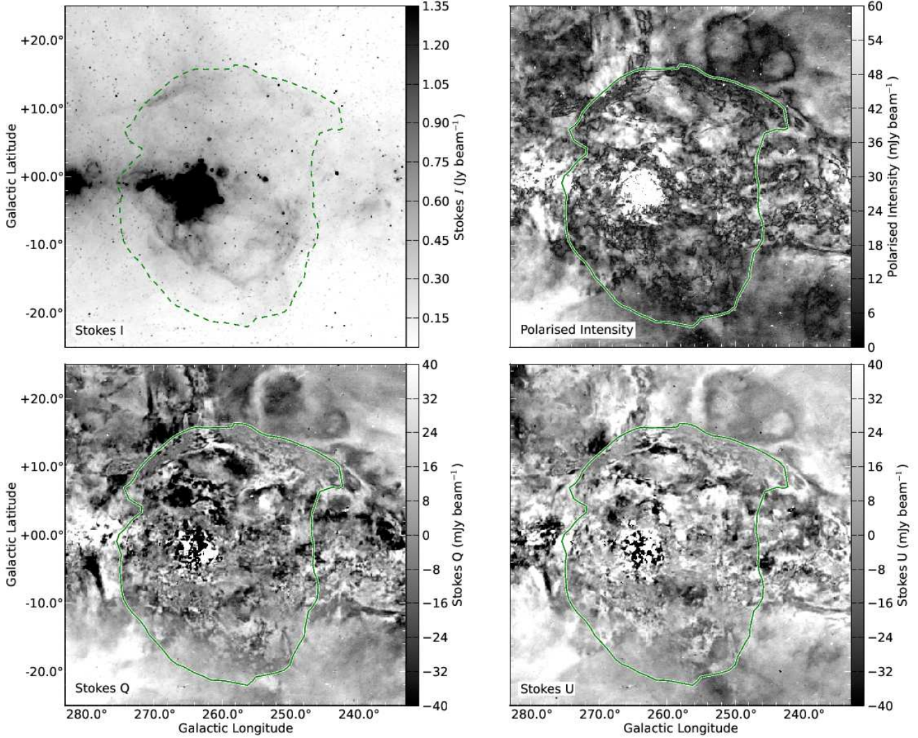
Fig. 5.— 2.3 GHz radio-continuum maps of the Gum Nebula from the S-PASS project. The data are calibrated in Janskys and may be converted to a main-beam brightness temperature scale in Kelvin by multiplying by 0.55. The border of the nebula traced by the green line is the same as in Fig. 2.
