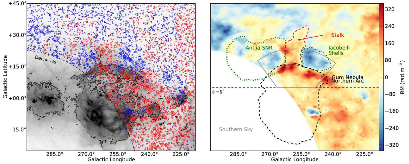
Fig. 2.— Left : The RM-catalogue of Taylor et al. (2009) plotted over the H\alpha map of the Gum Nebula (Finkbeiner 2003). Red circles indicate positive RMs, while blue indicate negative and their diameter is proportional to |RM| . The solid H\alpha contour at a level of 25 R defines the outline of the nebula. Right : Prominent RM-features are easier to visualise in the map produced by Oppermann et al. (2012) using the Taylor et al. (2009) catalogue. Polygons and lines annotate significant features. We restrict our analysis to the upper arc region, inside the solid grey line.
