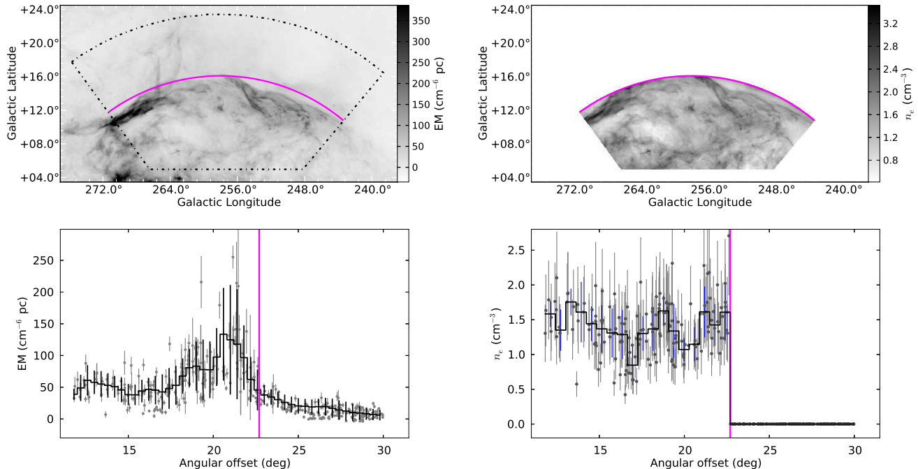
Fig. 8.— Left : EM map and azimuthally averaged profile of the upper Gum region. The individual grey points in the bottom panel show the EM values at the positions of the RM samples while the black points with error bars show the azimuthal average and standard-deviation in 0.2 degree bins. Right : Electron density map and azimuthally averaged profile derived assuming the best-fit parameters in Table 2. The magenta line shows the edge of the shell model.
