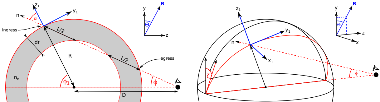
Fig. 16.— Geometry of an ionised shell in the near-field. We assume a constant electron density n_e in the shell, which is threaded with a uniform magnetic field. The field is confined to the y - z plane, representing the Galactic disk, and only the sky pitch-angle \Theta may be varied.
