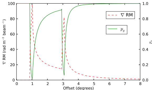
Fig. 15.— The depolarising effect of the spatial gradient in RM at the inner and outer edge of an ionised shell. The dotted/red line shows the gradient in rotation measure ( dRM/dr ) in units of \text{rad m}^{-2} \text{beam}^{-1} as a function of position, crossing the shell from outside to the interior. The solid/green line shows the corresponding degree of polarisation calculated from Equation 17.
