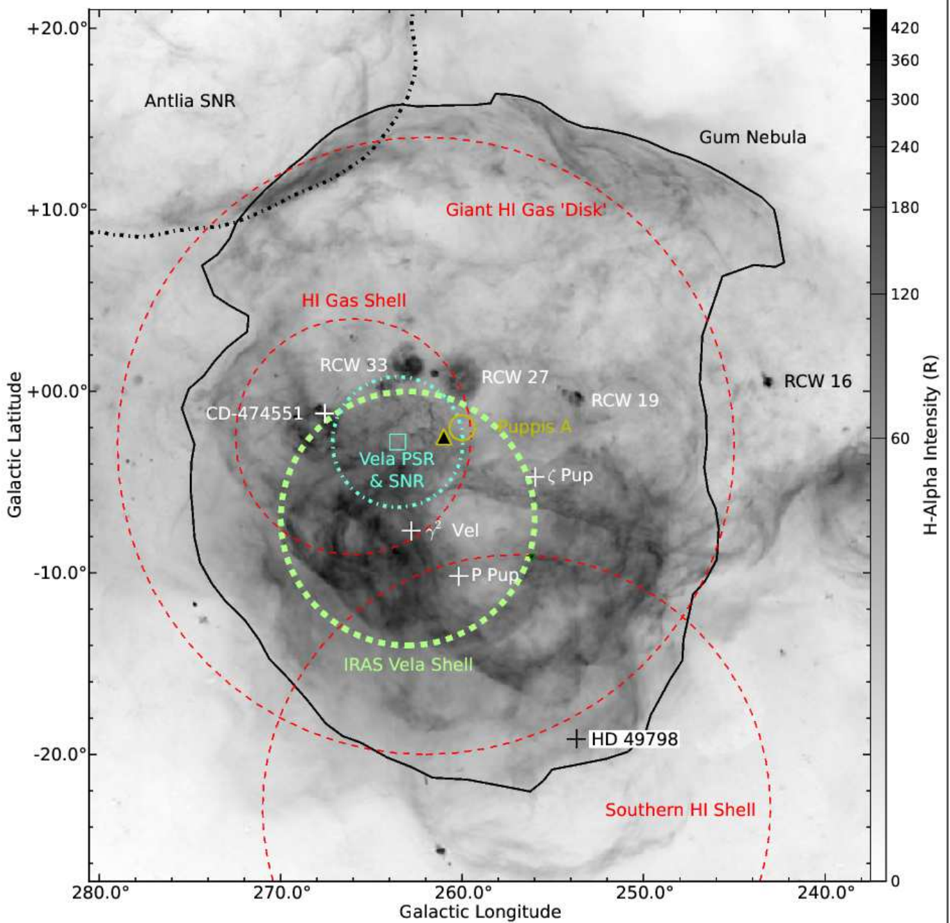
Fig. 1.— An H \alpha image of the Gum Nebula (Finkbeiner 2003) annotated with significant objects identified in the literature. OB-type stars are marked with ‘+’ symbols, the Vela pulsar with a square and the kinematic centre of the nebula derived by Woermann et al. (2001) with a triangle. Boundaries of gas-disks or shells are marked using coloured circles. See §1.1 for details. References for the annotated objects are as follows: Antlia SNR: McCullough et al. 2002; Giant H I Gas Disk: Reynoso & Dubner 1997; H I Gas Shell: Dubner et al. 1992; IRAS Vela Shell: Sahu & Sahu 1993; RCW-H II regions: Rodgers et al. 1960; Vela Pulsar: Radhakrishnan & Manchester 1969; CD-474551: Reed 2003; HD 49798 and \zeta Puppis: van Leeuwen 2007; \gamma^2 Velorum: De Marco & Schmutz 1999.
