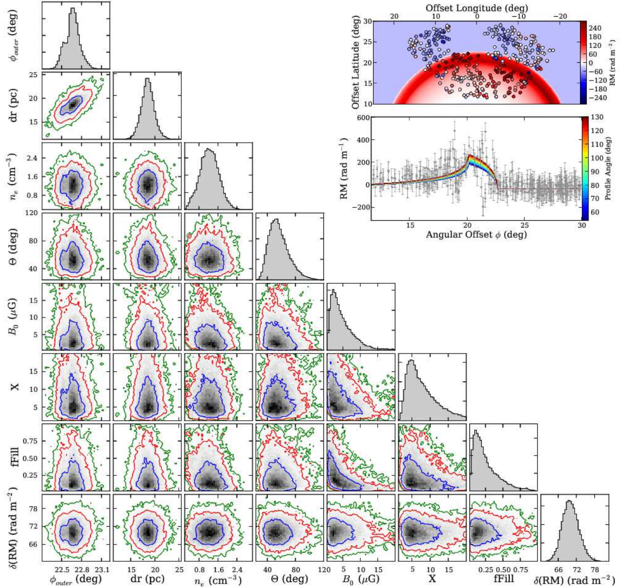
Fig. 11.— As for Fig. 9, but assuming a background as given by Jansson & Farrar (2012).
