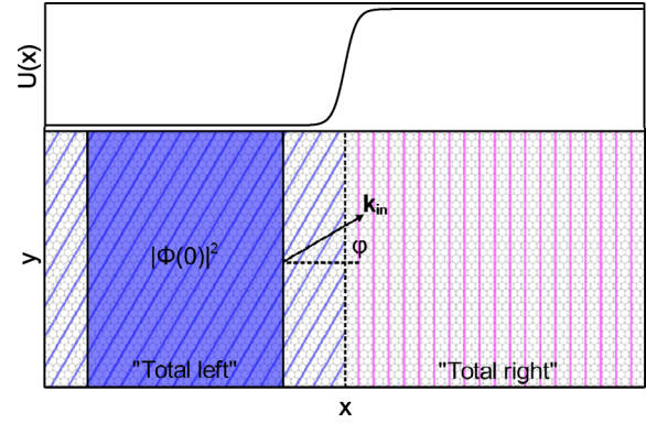
FIG. 3. (Color online) Simulation setup for n-p and n-n' junctions. The junction is located at the center. The areas for which the density is calculated cover the whole lattice. After the whole wave packet is either reflected or transmitted at the junction, the reflection and transmission are obtained. To prevent interference at the borders, a spacing between the initial wave packet and the left edge is introduced.
