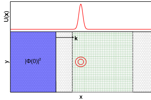
FIG. 10. (Color online) Setup of the simulation. The Gaussian potential is located at the center of the lattice and is indicated by two red circles. The initial wave packet is localized on the left of the lattice and is indicated in blue. The wave propagation is stored for the green (squared) area.
