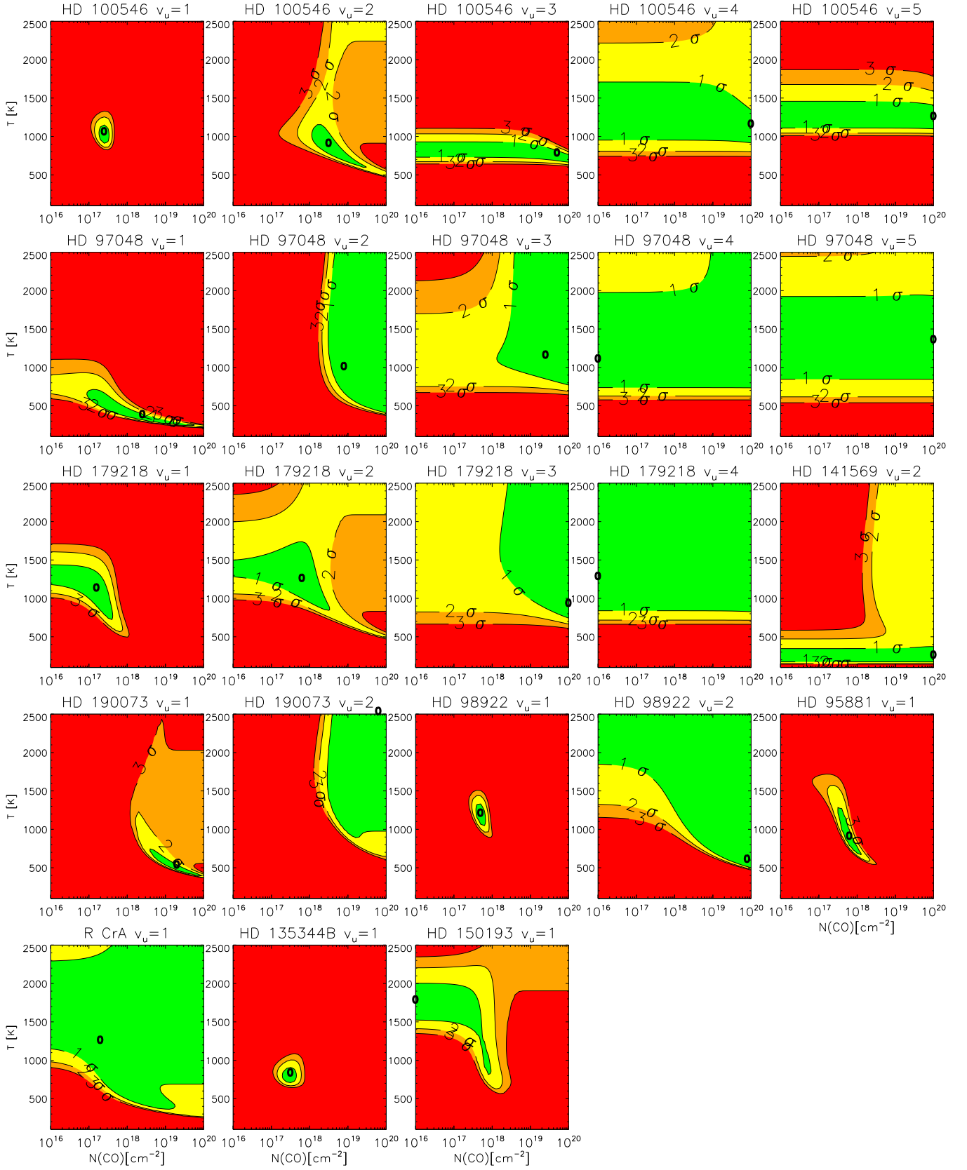
Fig. A.1: best fit contours for associated ^{12}\text{CO} Boltzmann plots. Color contours denote deviations of 1\sigma (green), 2\sigma (yellow), 3\sigma (orange) and > 3\sigma (red) confidence intervals
