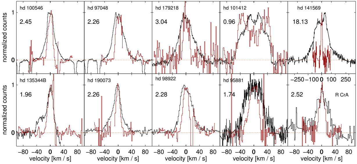
Fig. 9: 6300 \text{ \AA} [O I] emission (black histograms), and CO v = 1-0 J \leq 15 average line profiles (red lines), together with their 10% width [O I]/CO ratio. The CO emission of HD 141569 is averaged over the v = 2-1 lines, and because of problems with the telluric correction, we have used the high ( J_u \geq 30 ) for R CrA and HD 150193. The CO line profile plotted for HD 101412 is a blend of the ^{13}\text{CO } v = 1-0 R(23) and the ^{12}\text{CO } v = 4-3 R(35) lines. We show [O I] data of HD 97048 and HD 100546 from Acke & van den Ancker (2006), of HD 101412, HD 135344B, and HD 179218 from van der Plas et al. (2008), of HD 190073 from R. van Lieshout and T. Bagnoli (private communication; HERMES spectrograph at the Mercator telescope), and from Acke et al. (2005) for the other stars. We note that both the CO and [O I] lines have been centered at 0 velocity, and the differing velocity scale for HD 141569.
