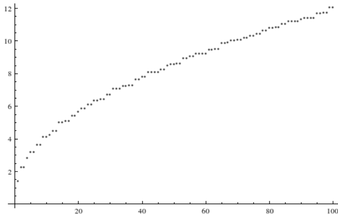
Figure 3 List of the eigenvalues of D_{\mathbb{T}^2} .
