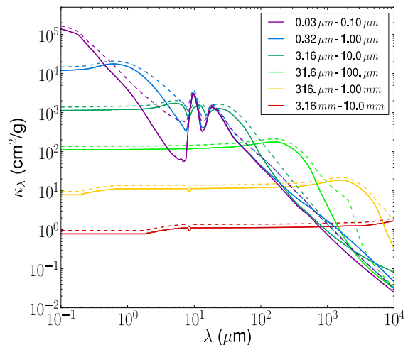
Fig. 6: The mass absorption (left) and total extinction (right) coefficients of the mixtures used in this work. Our 'standard' mixture (the full lines) contains 15% metallic iron, while the alternative mixture (the dashed lines) has 15% amorphous carbon instead. The latter composition is exactly the same as used by Mulders & Dominik (2012). Only six grain sizes are shown for clarity.
