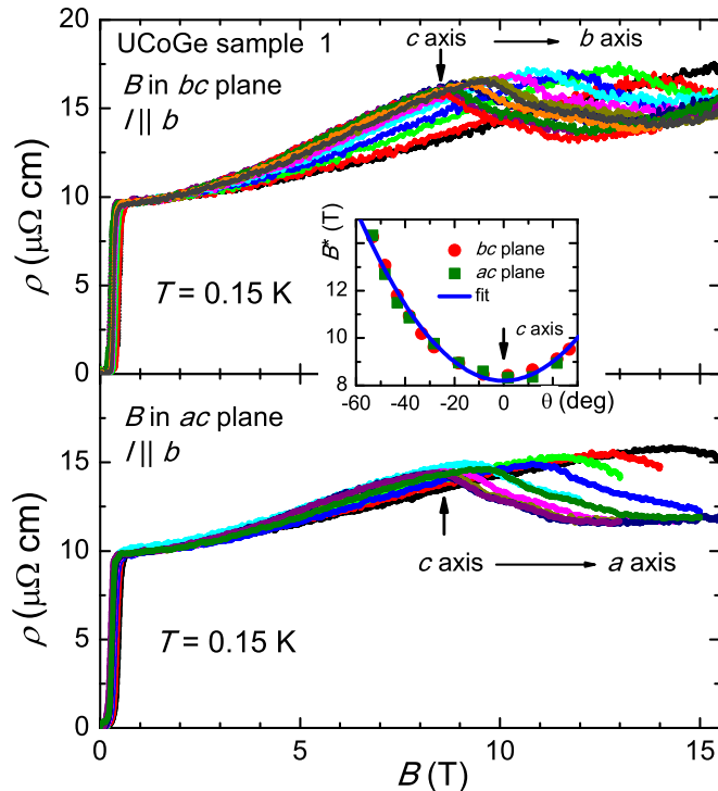
FIG. 2. (Color online) Angular variation of the magnetoresistance of UCoGe (sample 1) at T = 0.15 K. The top panel shows the field rotation in the bc plane; \theta = -58^\circ, -53^\circ, -48^\circ, -43^\circ, -38^\circ, -33^\circ, -28^\circ, -18^\circ, -8^\circ, 2^\circ, 12^\circ, 22^\circ, and 27^\circ , where 0^\circ corresponds to B \parallel c . The lower panel shows the field rotation in the ac plane; \theta = -53^\circ, -48^\circ, -43^\circ, -38^\circ, -28^\circ, -18^\circ, -8^\circ, 2^\circ, 12^\circ, 22^\circ, and 27^\circ . The current is always applied along the b axis. The inset shows B^* as a function of \theta . The solid line represents B^*(\theta) = B^*(0)/\cos \theta .
