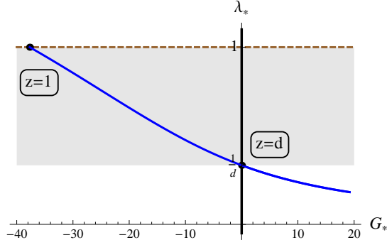
Figure 1: z -dependence of the fixed point arising from (13). The dashed horizontal line represents the general relativistic case, while the thick vertical line represents the line of Gaussian fixed points. In the shaded area the extra scalar mode of HL gravity is classically unstable [10].
