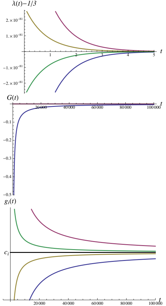
Figure 2: Scale-dependence of the wave-function renormalizations G_k and \lambda_k and the marginal couplings \tilde{g}_i in d = z = 3 . The aGFP (19,21) acts as a UV attractor of the RG flow.
