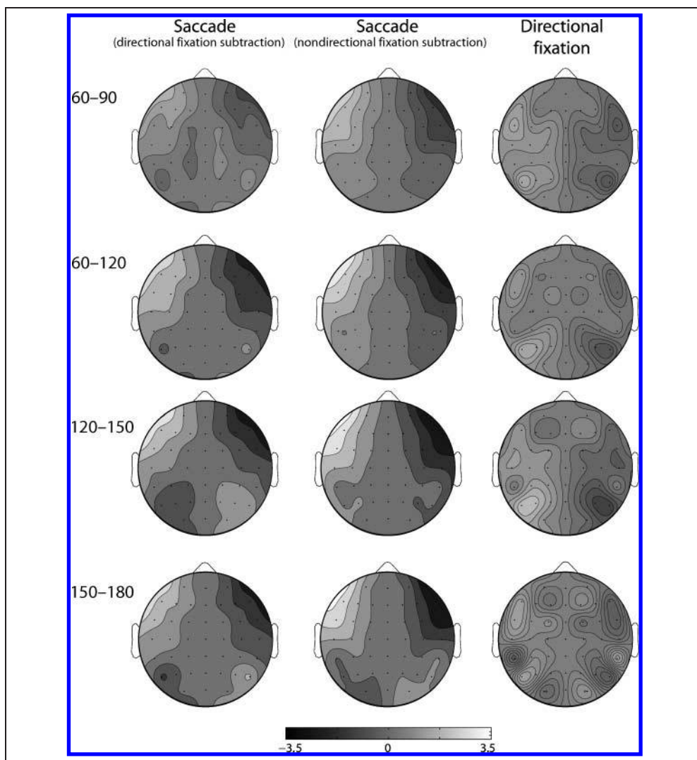
Figure 4. Double subtraction EEG topoplots for the saccade and directional fixation conditions for different time windows. To obtain the double subtraction plots, activity from the left and right hemispheres was subtracted for both conditions, and the resulting activity maps were subtracted again (saccade/cue-left minus saccade/cue-right). Activity in the left hemisphere reflects contralateral activity. Because of this subtraction, only lateralized activity is visible. Shown are plots for the saccade condition, with directional fixation subtracted (left); the saccade condition with nondirectional fixation subtracted (center) and the directional fixation condition with nondirectional fixation as baseline. Plots are averaged over the entire time window.
