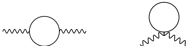
Figure 2. Diagrammatic representation of the two terms in the r.h.s. of the flow equation (3.16) for the c -function.
