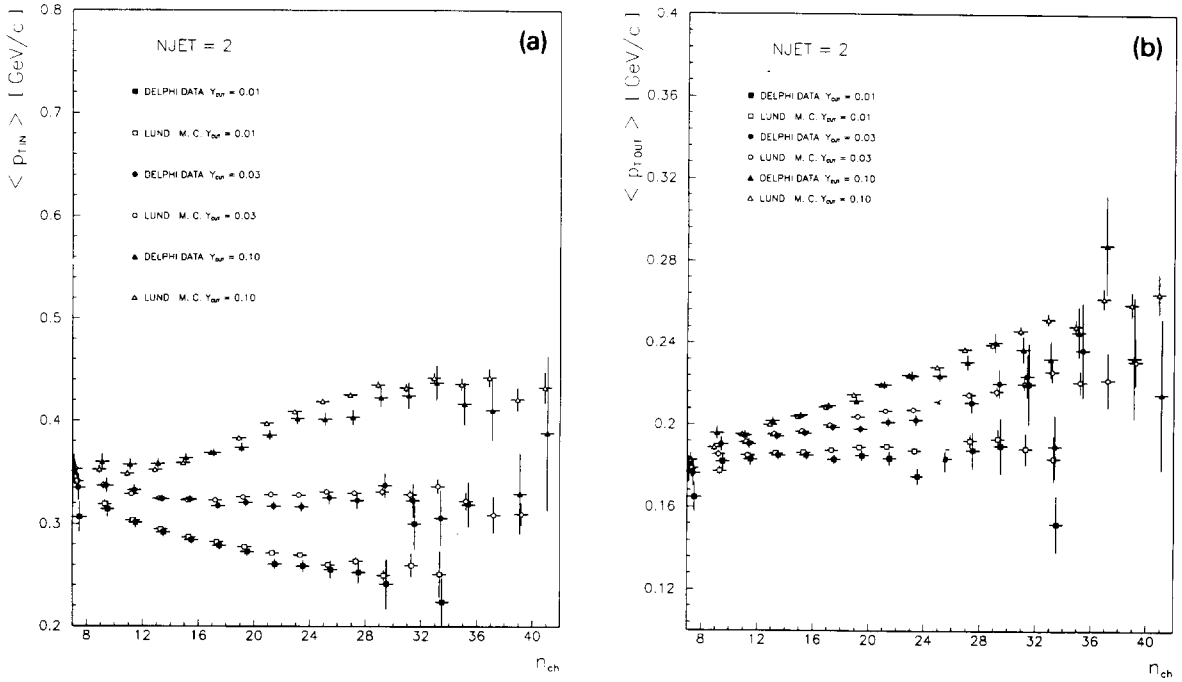
Fig. 4. Dependence, (a) of \langle p_{t,in} \rangle , (b) of \langle p_{t,out} \rangle , on n_{ch} , shown for events in 2-jet samples defined with different choices of the y_{CUT} parameter: y_{CUT} = 0.01, 0.03, 0.10 . The data are compared with the predictions of the Lund Parton Shower model.
