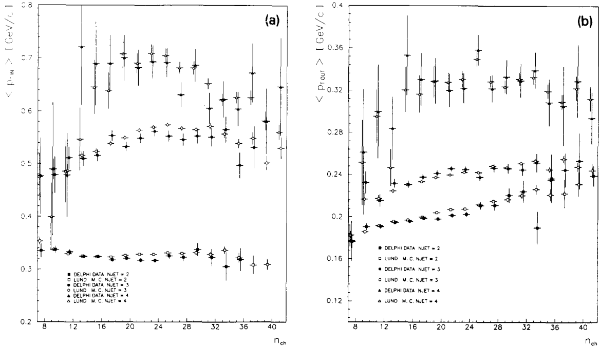
Fig. 3. Dependence, (a) of \langle p_{t,in} \rangle , (b) of \langle p_{t,out} \rangle , on n_{ch} , shown for events with different numbers of jets, NJET = 2, 3, 4. The data are compared with the predictions of the Lund Parton Shower model.
