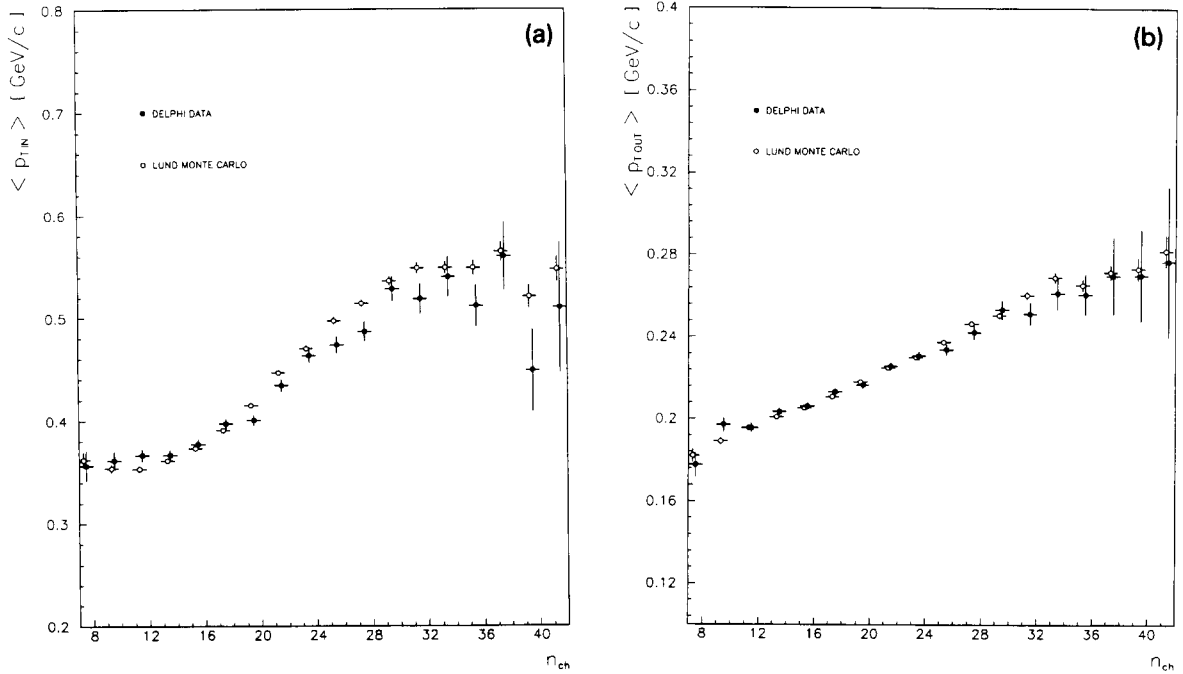
Fig. 1. Dependence of mean transverse momenta in the event plane - \langle p_{t,in} \rangle (a), and in the direction perpendicular to the event plane - \langle p_{t,out} \rangle (b), on charged particle multiplicity in e^+e^- annihilations into hadrons at \sqrt{s}=91 GeV. The data are compared with the predictions of the Lund Parton Shower model.
