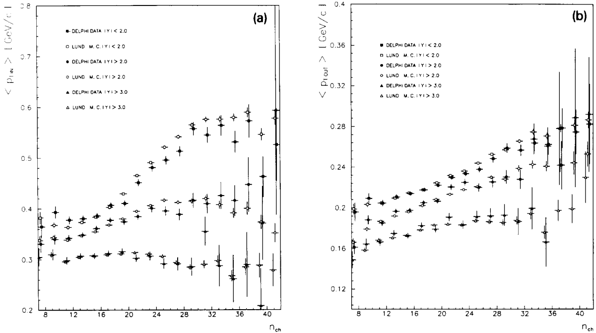
Fig. 2. Dependence, (a) of \langle p_{t,in} \rangle , (b) of \langle p_{t,out} \rangle , on n_{ch} , shown for three regions of rapidity: a central region |y| < 2.0 and two outer regions |y| > 2.0 and |y| > 3.0 . The data are compared with the predictions of the Lund Parton Shower model.
