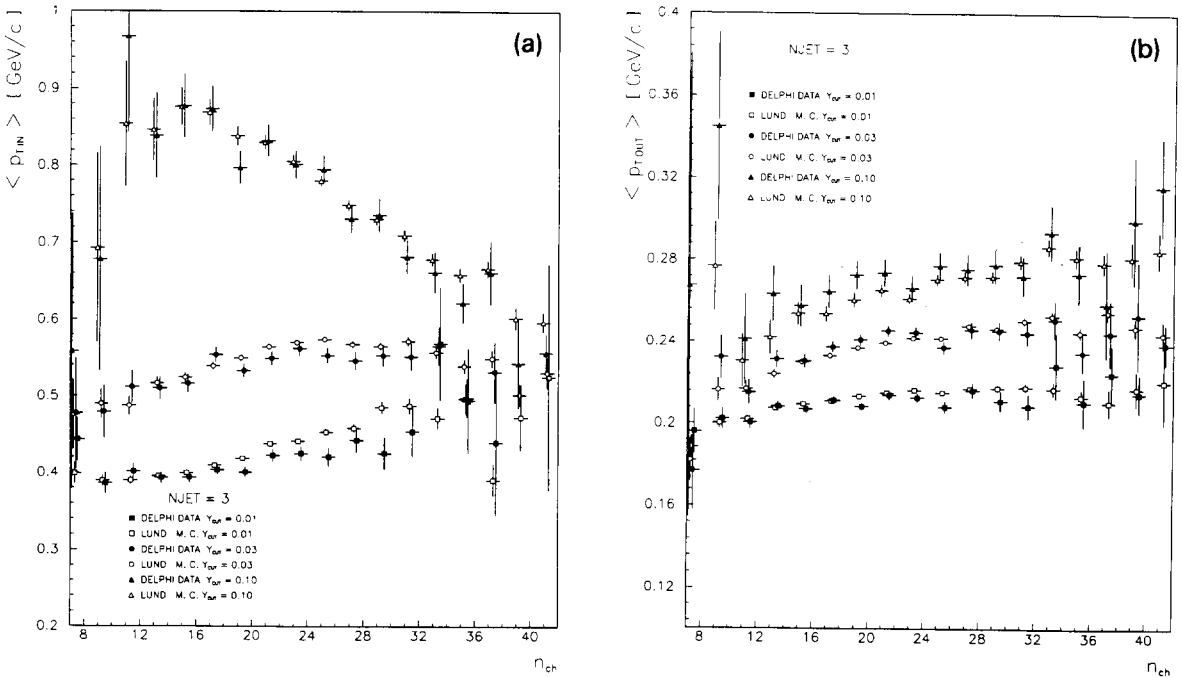
Fig. 5. Dependence, (a) of \langle p_{t,in} \rangle , (b) of \langle p_{t,out} \rangle , on n_{ch} , shown for events in 3-jet samples defined with different choices of the y_{CUT} parameter: y_{CUT} = 0.01, 0.03, 0.10 . The data are compared with the predictions of the Lund Parton Shower model.
