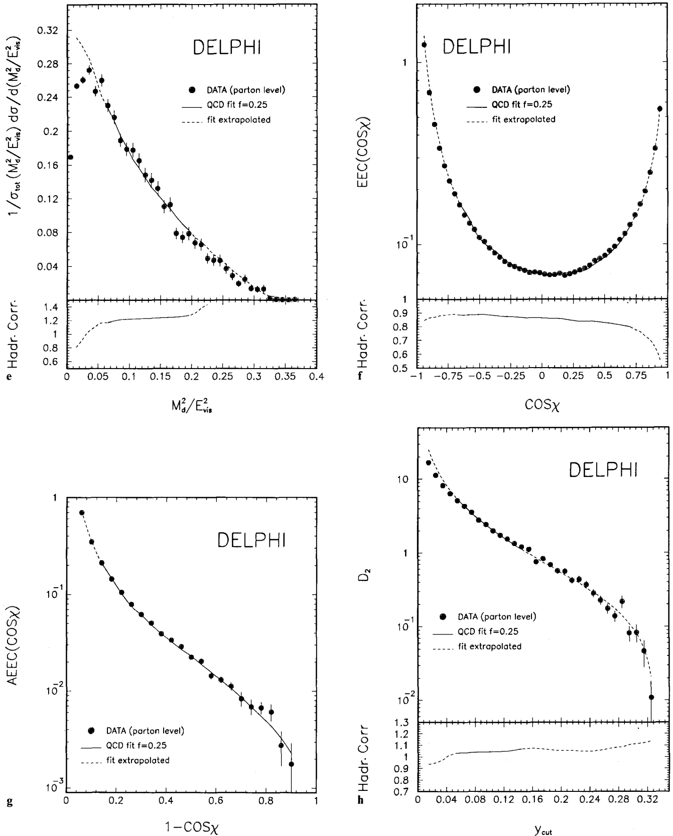
Fig. 2a-h. Experimental bare parton distributions of the thrust T (a), the oblateness O (b), the C -parameter C (c), the heavy mass M_h^2/E_{vis}^2 (d), the difference of the heavy and light mass M_d^2/E_{vis}^2 (e), the energy-energy correlation EEC (f) and its asymmetry AEEC (g) and the differential 2-jet rate D_2 (h). The errors shown contain
