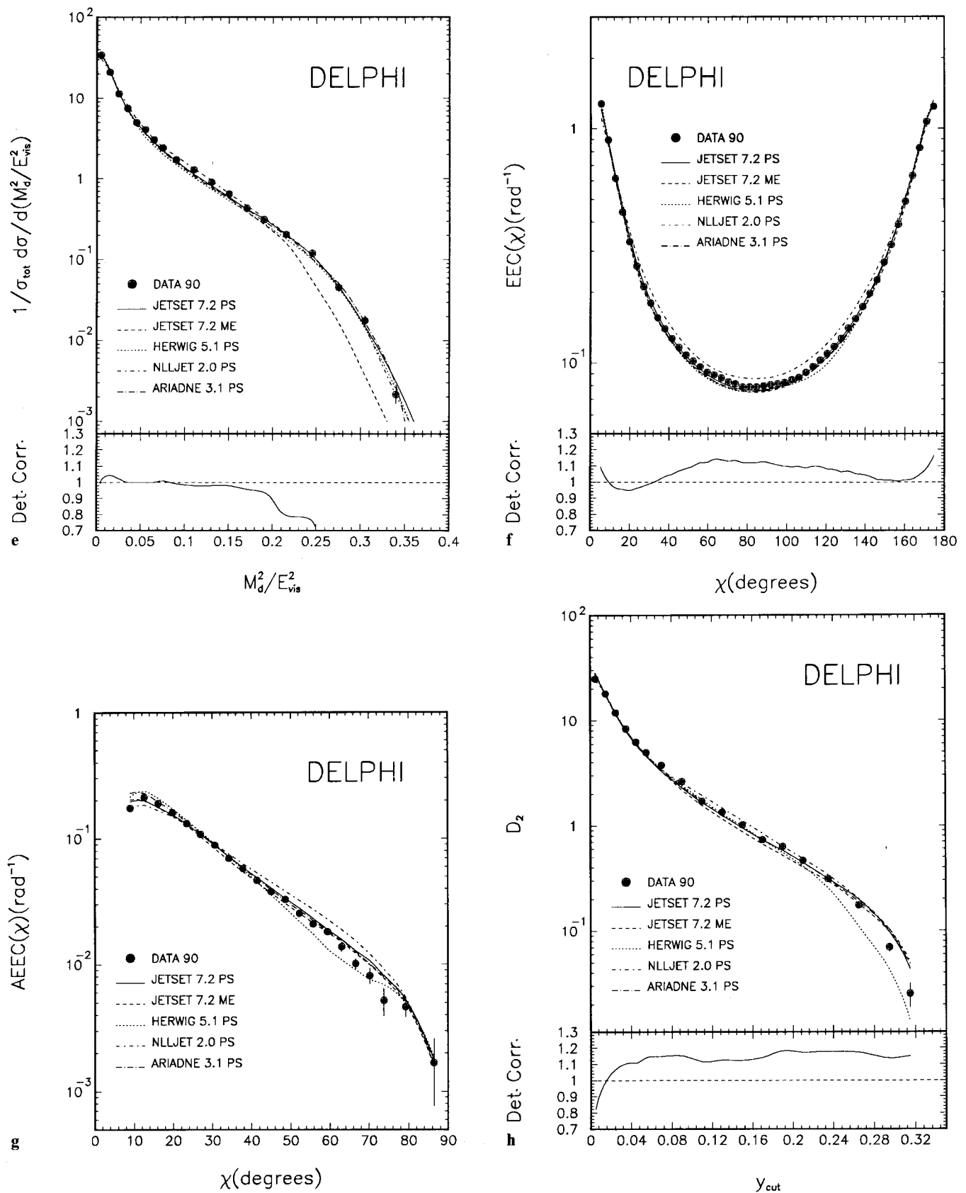
Fig. 1a-h. Experimental differential distributions of the thrust T (a), the oblateness O (b), the C -parameter C (c), the heavy mass M_d^2/E_{\text{vis}}^2 (d), the difference of the heavy and light mass M_d^2/E_{\text{vis}}^2 (e), the energy-energy correlation \text{EEC} (f) and its asymmetry \text{AEEC} (g) and the differential 2-jet rate D_2 (h) in comparison to the pre-
