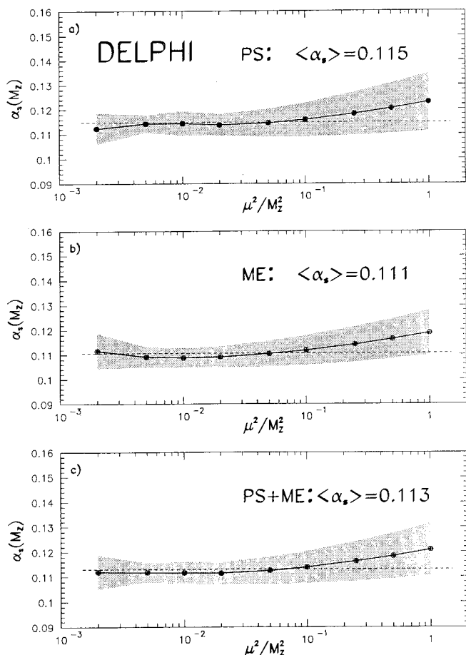
Fig. 4a-c. Averaged values of \alpha_s(M_Z) at different scales of \mu^2/M_Z^2 for hadronization corrections done with the JETSET 7.2 PS model (a) and with the JETSET 7.2 ME model (b). The error-bands shown indicate the disagreement between the \alpha_s values obtained from the different observables due to missing higher order corrections in the theoretical calculations
