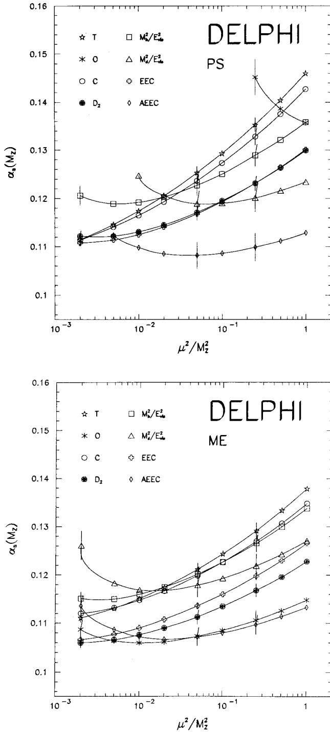
Fig. 3a, b. Values of \alpha_s(M_Z) at different scales of \mu^2/M_Z^2 for the distributions thrust T , oblateness O , C -parameter C , heavy mass M_h^2/E_{\text{vis}}^2 , difference of the heavy and light mass M_l^2/E_{\text{vis}}^2 , energy-energy correlation EEC and its asymmetry AEEC and the differential 2-jet rate D_2 . The errors show some typical statistical and experimental systematic errors added in quadrature. The hadronization corrections are done with the JETSET 7.2 PS model in (a). The hadronization corrections are done with the JETSET 7.2 ME model in (b)
