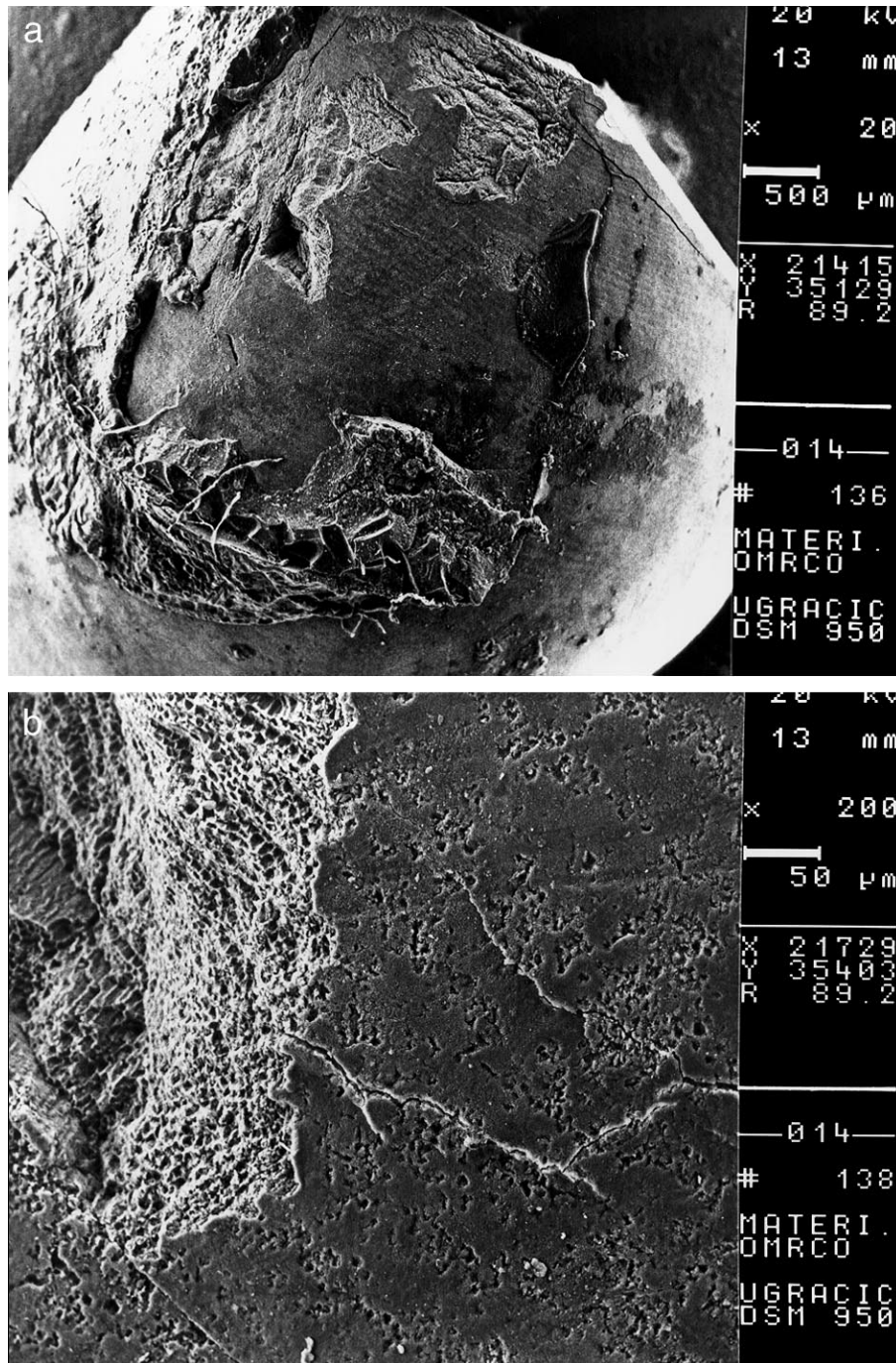
FIGURE 2. Specimen bonded with chemical-cured composite resin (System One). (a) A type III (mixed) failure may be observed. Cohesive failure of the enamel may also be observed (top-left) (20 \times magnification). (b) Higher magnification of the enamel morphology after debonding. Fractured enamel prisms and a porous enamel surfaces are shown (200 \times magnification).
