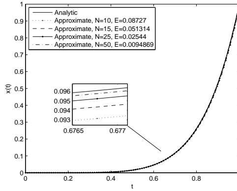
Figure 4: Example 2: analytic vs. numerical approximation.
