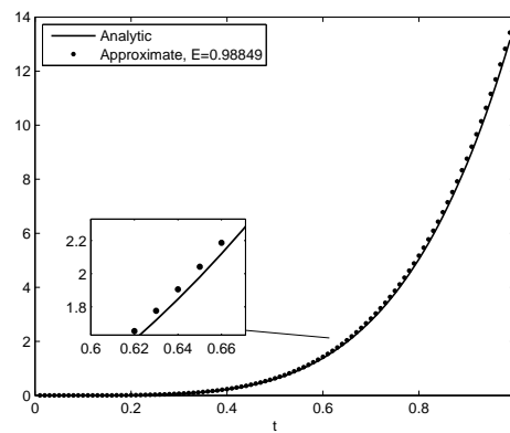
Figure 2: For N = 50 : analytic vs. numerical approximation.
